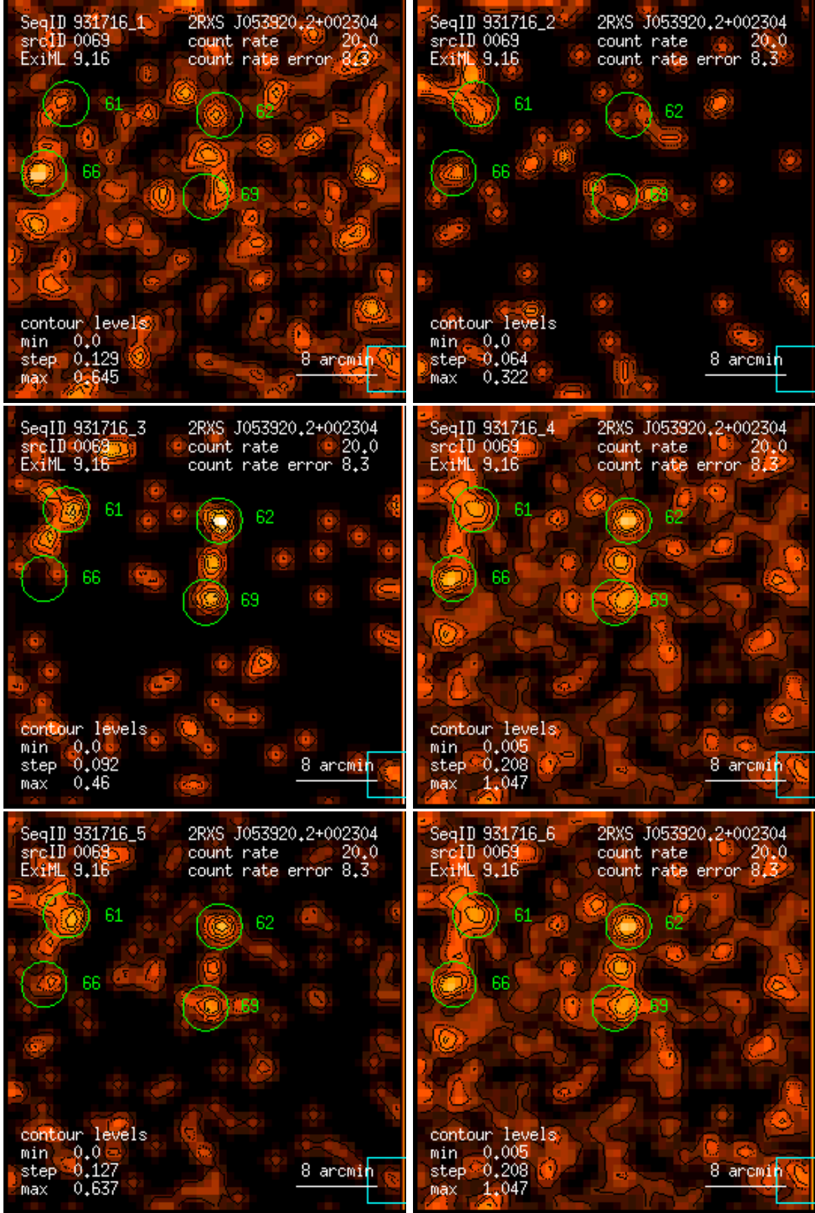
Figure 69: RASS 931716: detection 0069: band rate images, Gaussian filter: (1) PSPC channels 11 – 41, (2) 52 – 90, (3) 91 – 201, (4) 11 – 235, (5) 52 – 201, (6) 11 – 201. Broad band rates in counts/ks. Band rate contour levels in counts/ks/arcmin 2 .
