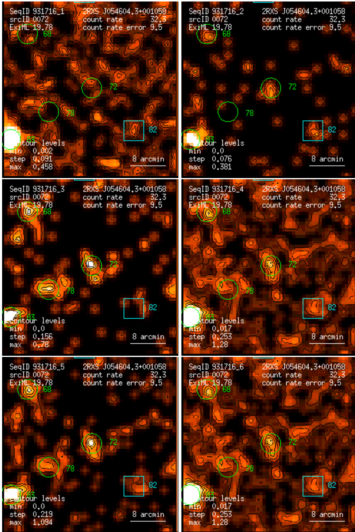
Figure 72: RASS 931716: detection 0072: band rate images, Gaussian filter: (1) PSPC channels 11 – 41, (2) 52 – 90, (3) 91 – 201, (4) 11 – 235, (5) 52 – 201, (6) 11 – 201. Broad band rates in counts/ks. Band rate contour levels in counts/ks/arcmin 2 .
