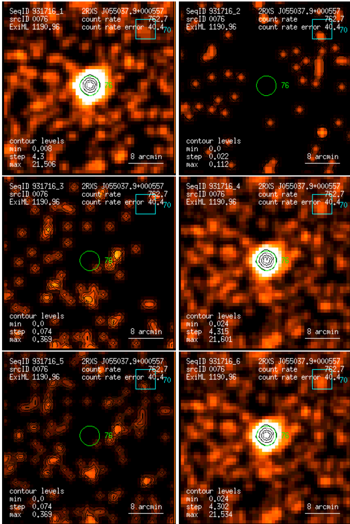
Figure 76: RASS 931716: detection 0076: band rate images, Gaussian filter: (1) PSPC channels 11 – 41, (2) 52 – 90, (3) 91 – 201, (4) 11 – 235, (5) 52 – 201, (6) 11 – 201. Broad band rates in counts/ks. Band rate contour levels in counts/ks/arcmin 2 .
