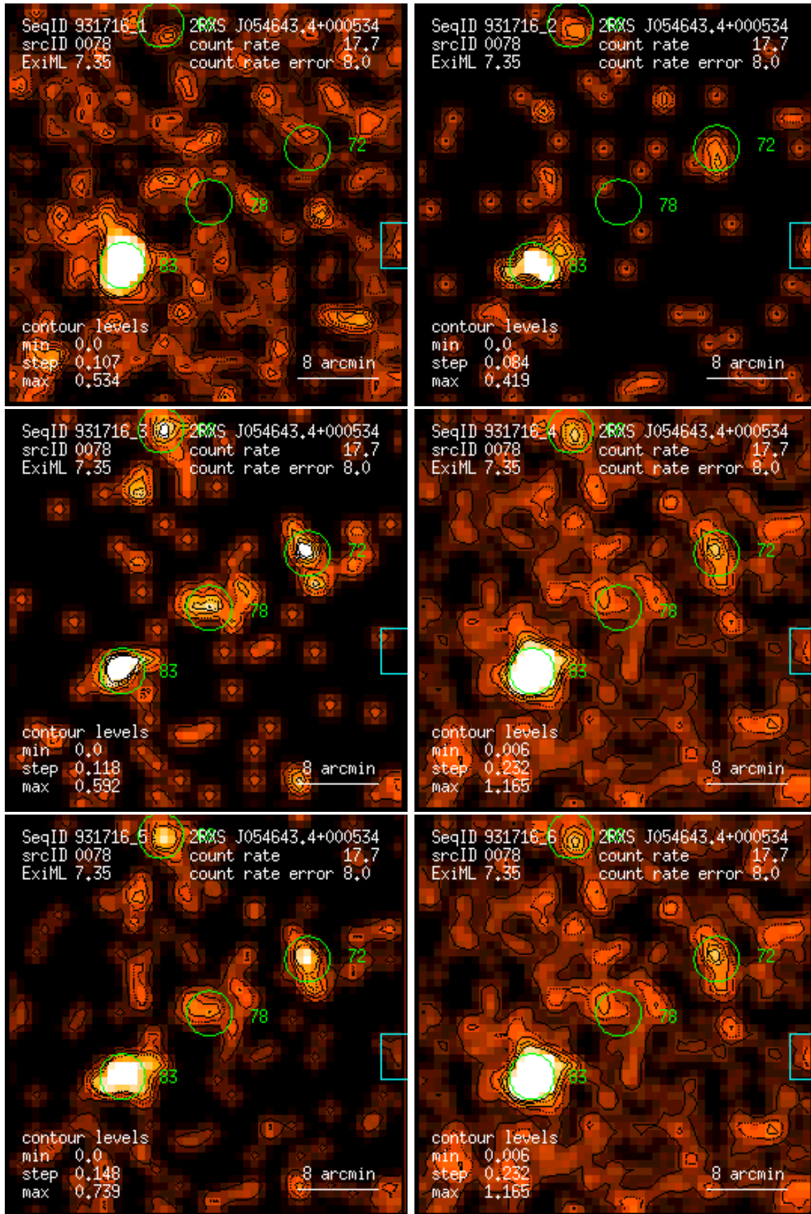
Figure 78: RASS 931716: detection 0078: band rate images, Gaussian filter: (1) PSPC channels 11 – 41, (2) 52 – 90, (3) 91 – 201, (4) 11 – 235, (5) 52 – 201, (6) 11 – 201. Broad band rates in counts/ks. Band rate contour levels in counts/ks/arcmin 2 .
