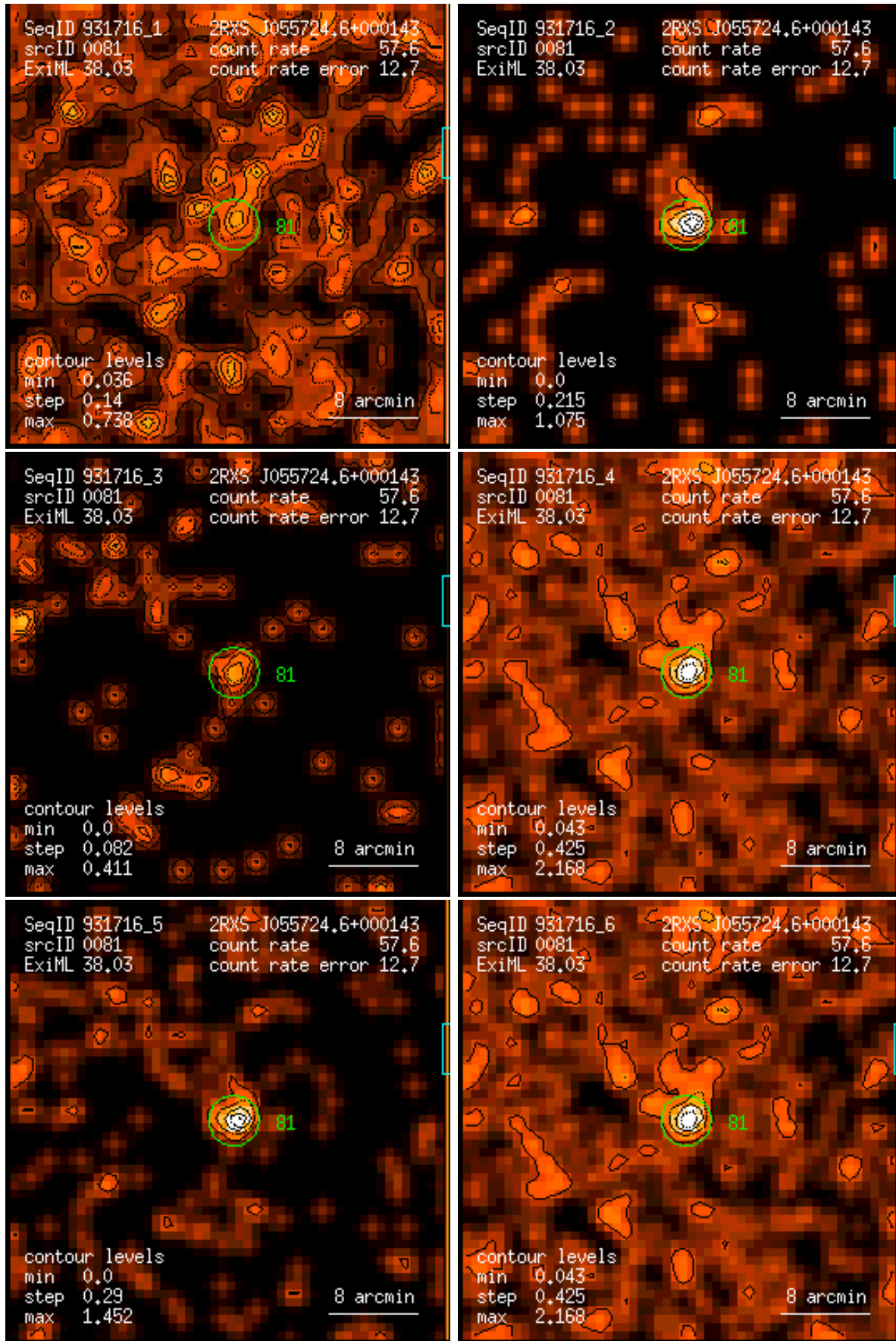
Figure 81: RASS 931716: detection 0081: band rate images, Gaussian filter: (1) PSPC channels 11 – 41, (2) 52 – 90, (3) 91 – 201, (4) 11 – 235, (5) 52 – 201, (6) 11 – 201. Broad band rates in counts/ks. Band rate contour levels in counts/ks/arcmin 2 .
