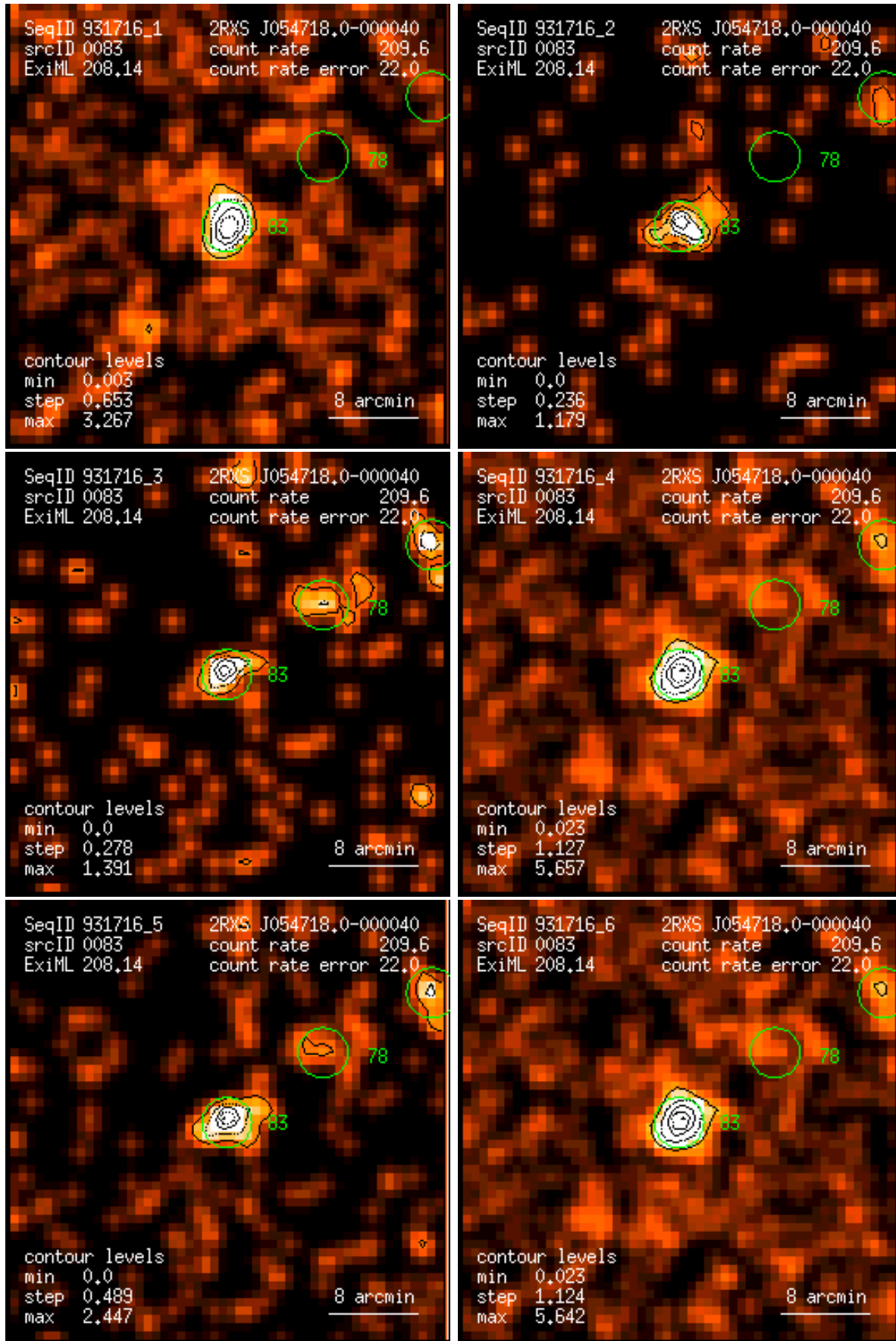
Figure 83: RASS 931716: detection 0083: band rate images, Gaussian filter: (1) PSPC channels 11 – 41, (2) 52 – 90, (3) 91 – 201, (4) 11 – 235, (5) 52 – 201, (6) 11 – 201. Broad band rates in counts/ks. Band rate contour levels in counts/ks/arcmin 2 .
