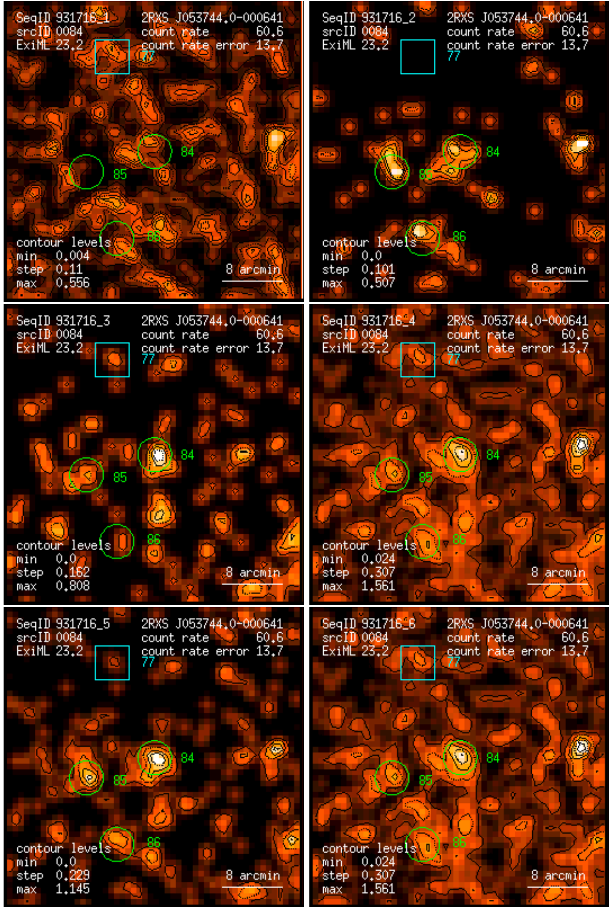
Figure 84: RASS 931716: detection 0084: band rate images, Gaussian filter: (1) PSPC channels 11 – 41, (2) 52 – 90, (3) 91 – 201, (4) 11 – 235, (5) 52 – 201, (6) 11 – 201. Broad band rates in counts/ks. Band rate contour levels in counts/ks/arcmin 2 .
