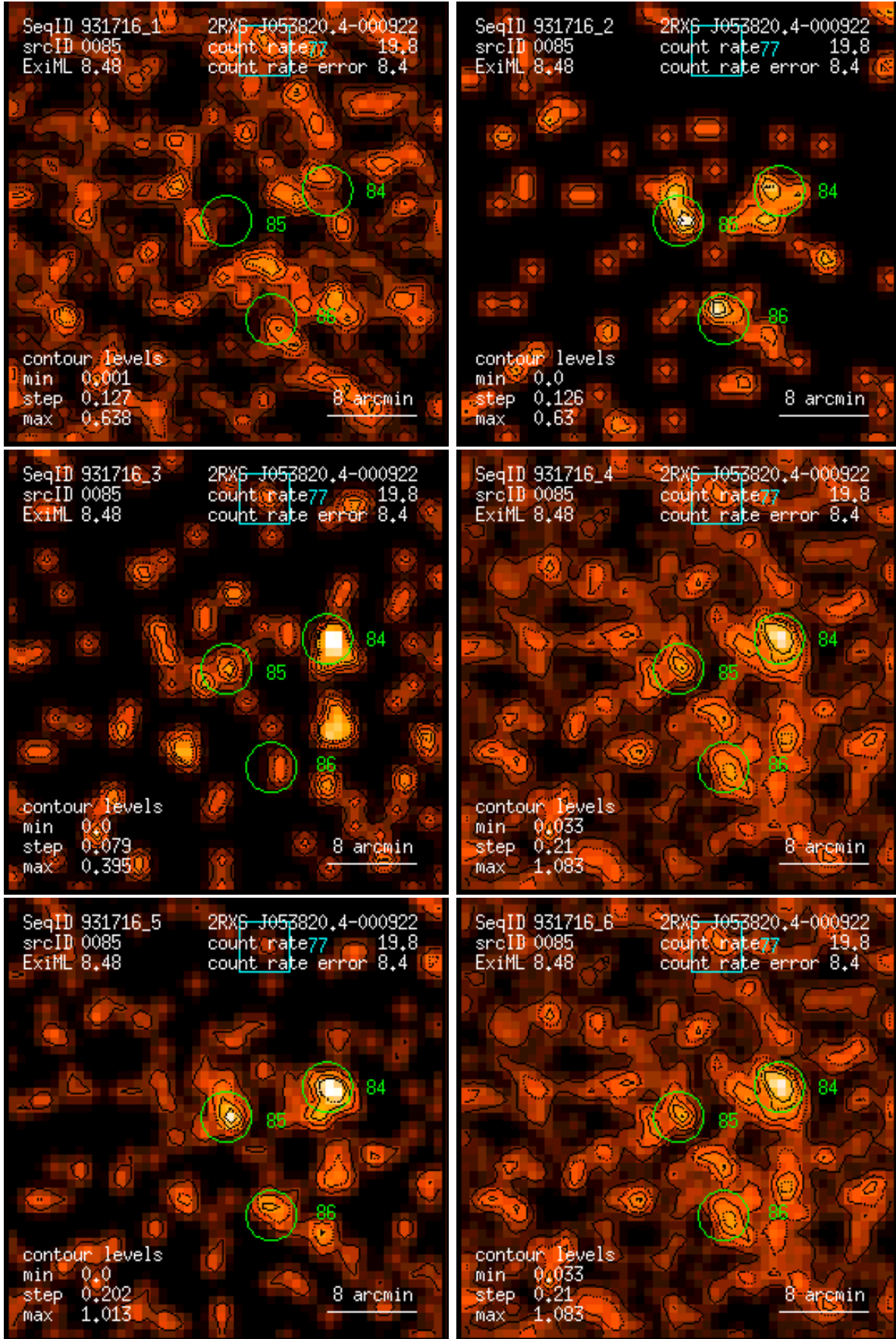
Figure 85: RASS 931716: detection 0085: band rate images, Gaussian filter: (1) PSPC channels 11 – 41, (2) 52 – 90, (3) 91 – 201, (4) 11 – 235, (5) 52 – 201, (6) 11 – 201. Broad band rates in counts/ks. Band rate contour levels in counts/ks/arcmin 2 .
