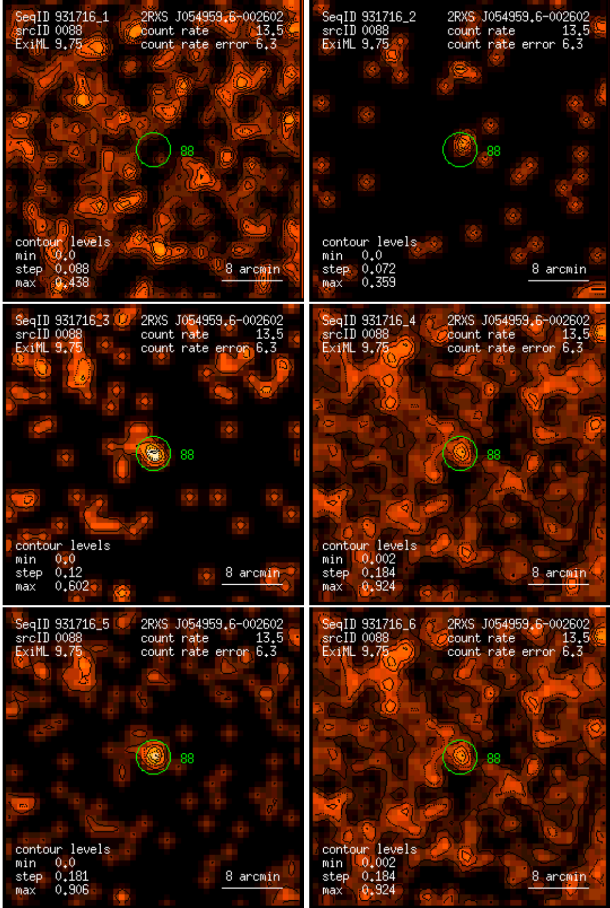
Figure 88: RASS 931716: detection 0088: band rate images, Gaussian filter: (1) PSPC channels 11 – 41, (2) 52 – 90, (3) 91 – 201, (4) 11 – 235, (5) 52 – 201, (6) 11 – 201. Broad band rates in counts/ks. Band rate contour levels in counts/ks/arcmin 2 .
