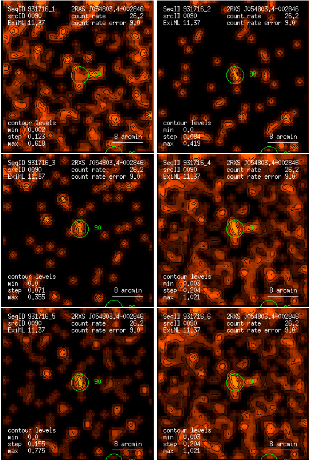
Figure 90: RASS 931716: detection 0090: band rate images, Gaussian filter: (1) PSPC channels 11 – 41, (2) 52 – 90, (3) 91 – 201, (4) 11 – 235, (5) 52 – 201, (6) 11 – 201. Broad band rates in counts/ks. Band rate contour levels in counts/ks/arcmin 2 .
