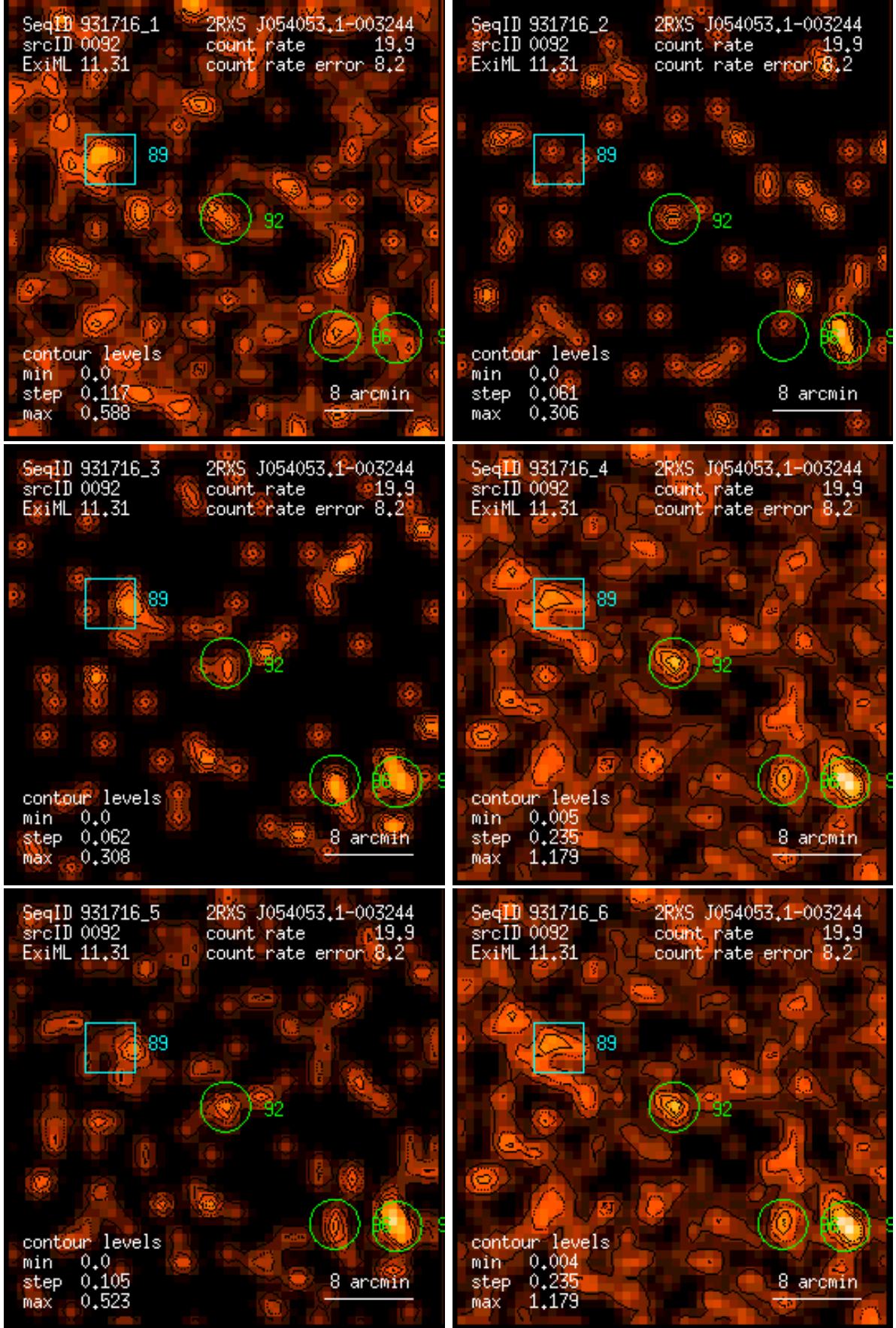
Figure 92: RASS 931716: detection 0092: band rate images, Gaussian filter: (1) PSPC channels 11 – 41, (2) 52 – 90, (3) 91 – 201, (4) 11 – 235, (5) 52 – 201, (6) 11 – 201. Broad band rates in counts/ks. Band rate contour levels in counts/ks/arcmin 2 .
