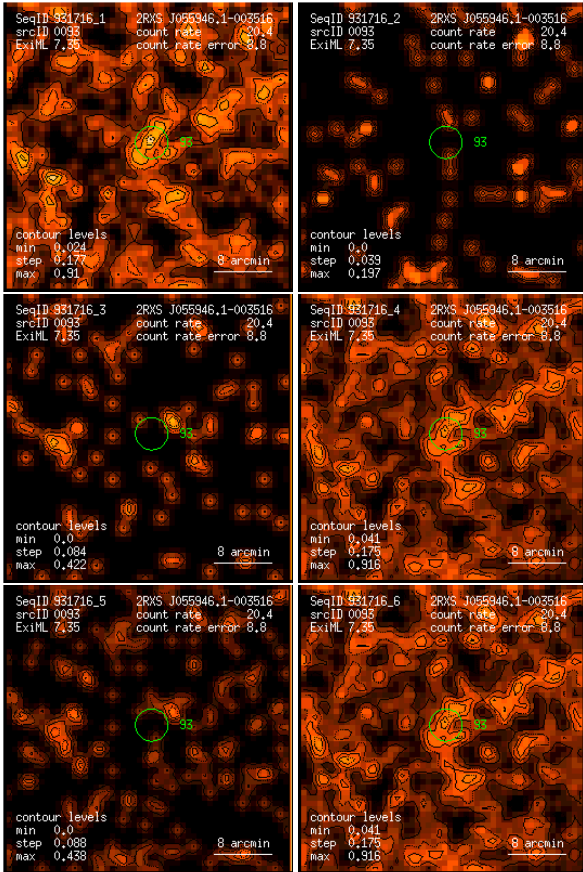
Figure 93: RASS 931716: detection 0093: band rate images, Gaussian filter: (1) PSPC channels 11 – 41, (2) 52 – 90, (3) 91 – 201, (4) 11 – 235, (5) 52 – 201, (6) 11 – 201. Broad band rates in counts/ks. Band rate contour levels in counts/ks/arcmin 2 .
