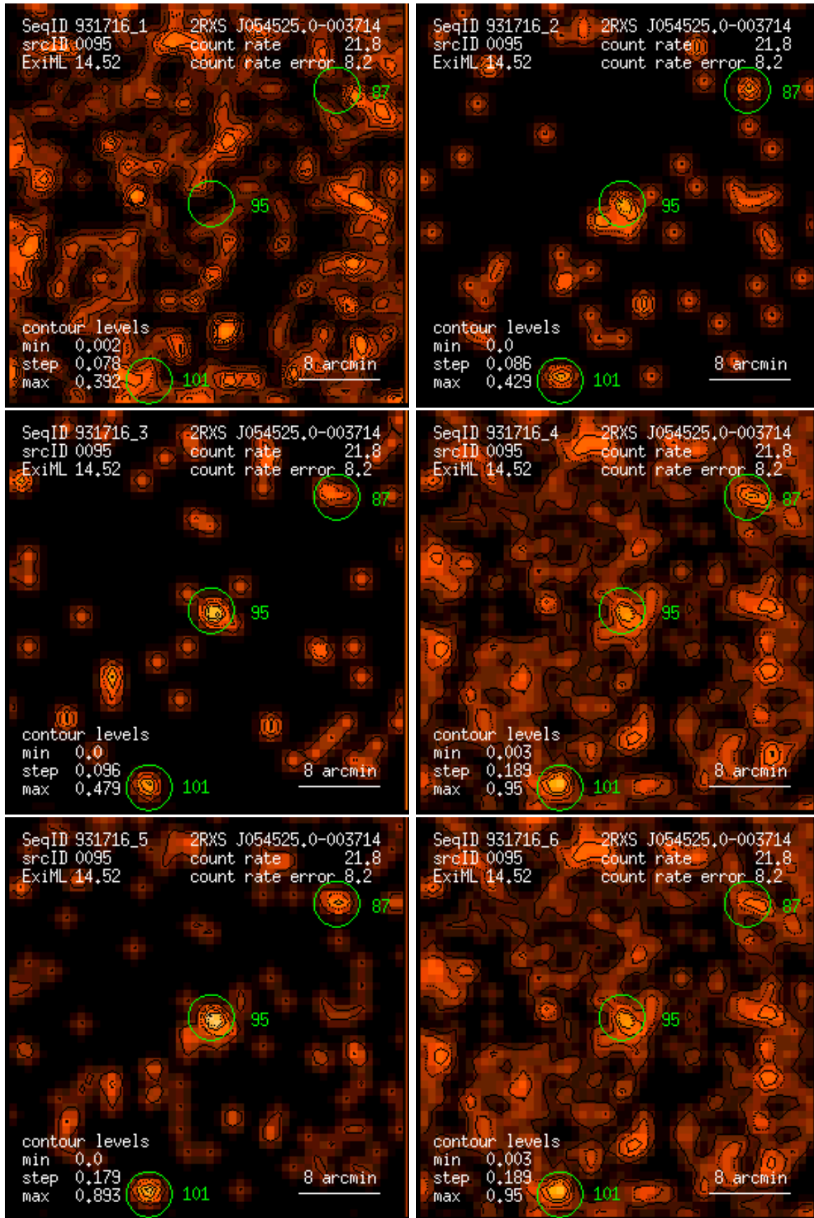
Figure 95: RASS 931716: detection 0095: band rate images, Gaussian filter: (1) PSPC channels 11 – 41, (2) 52 – 90, (3) 91 – 201, (4) 11 – 235, (5) 52 – 201, (6) 11 – 201. Broad band rates in counts/ks. Band rate contour levels in counts/ks/arcmin 2 .
