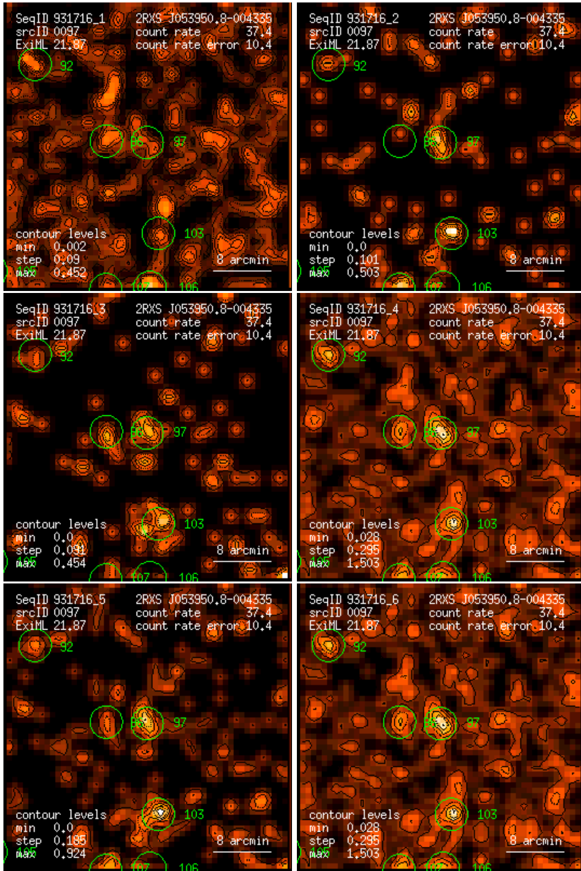
Figure 97: RASS 931716: detection 0097: band rate images, Gaussian filter: (1) PSPC channels 11 – 41, (2) 52 – 90, (3) 91 – 201, (4) 11 – 235, (5) 52 – 201, (6) 11 – 201. Broad band rates in counts/ks. Band rate contour levels in counts/ks/arcmin 2 .
