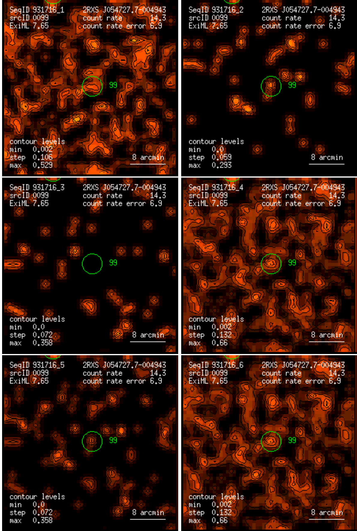
Figure 99: RASS 931716: detection 0099: band rate images, Gaussian filter: (1) PSPC channels 11 – 41, (2) 52 – 90, (3) 91 – 201, (4) 11 – 235, (5) 52 – 201, (6) 11 – 201. Broad band rates in counts/ks. Band rate contour levels in counts/ks/arcmin 2 .
