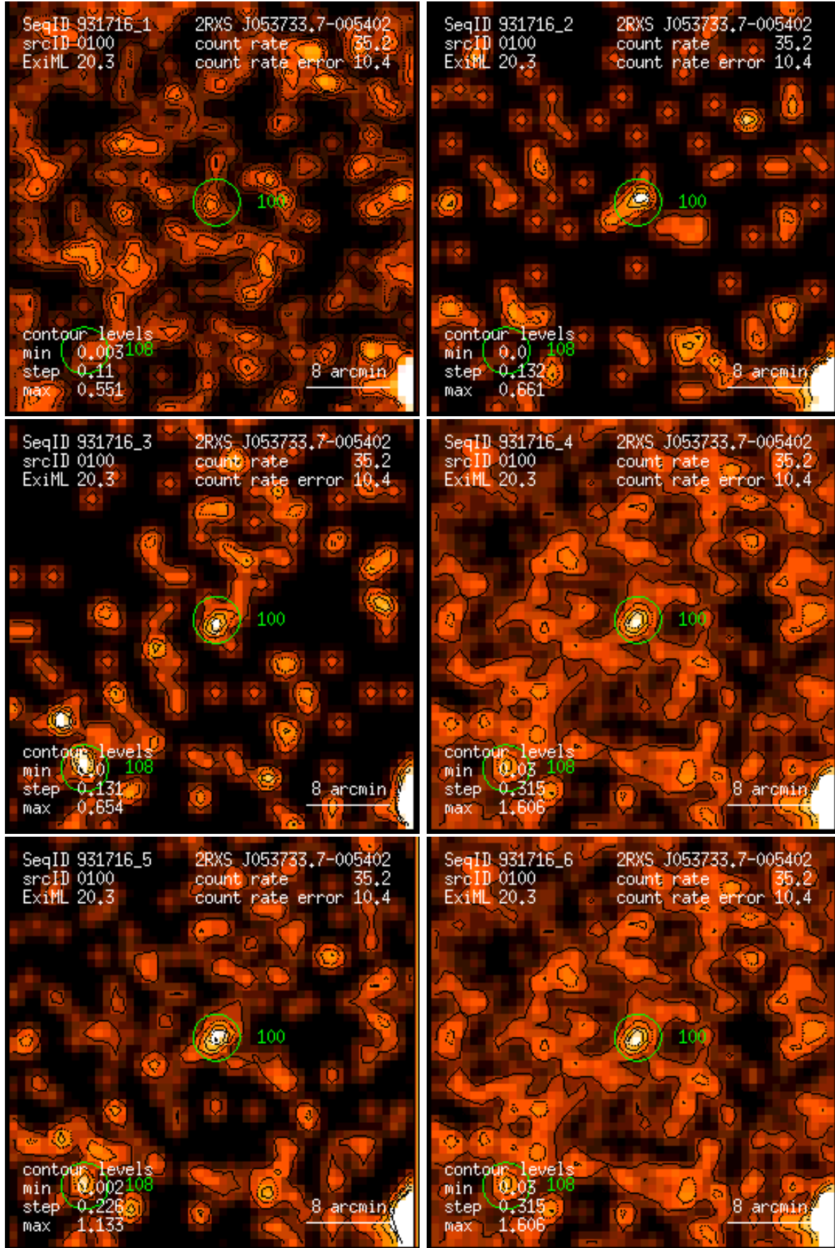
Figure 100: RASS 931716: detection 0100: band rate images, Gaussian filter: (1) PSPC channels 11 – 41, (2) 52 – 90, (3) 91 – 201, (4) 11 – 235, (5) 52 – 201, (6) 11 – 201. Broad band rates in counts/ks. Band rate contour levels in counts/ks/arcmin 2 .
