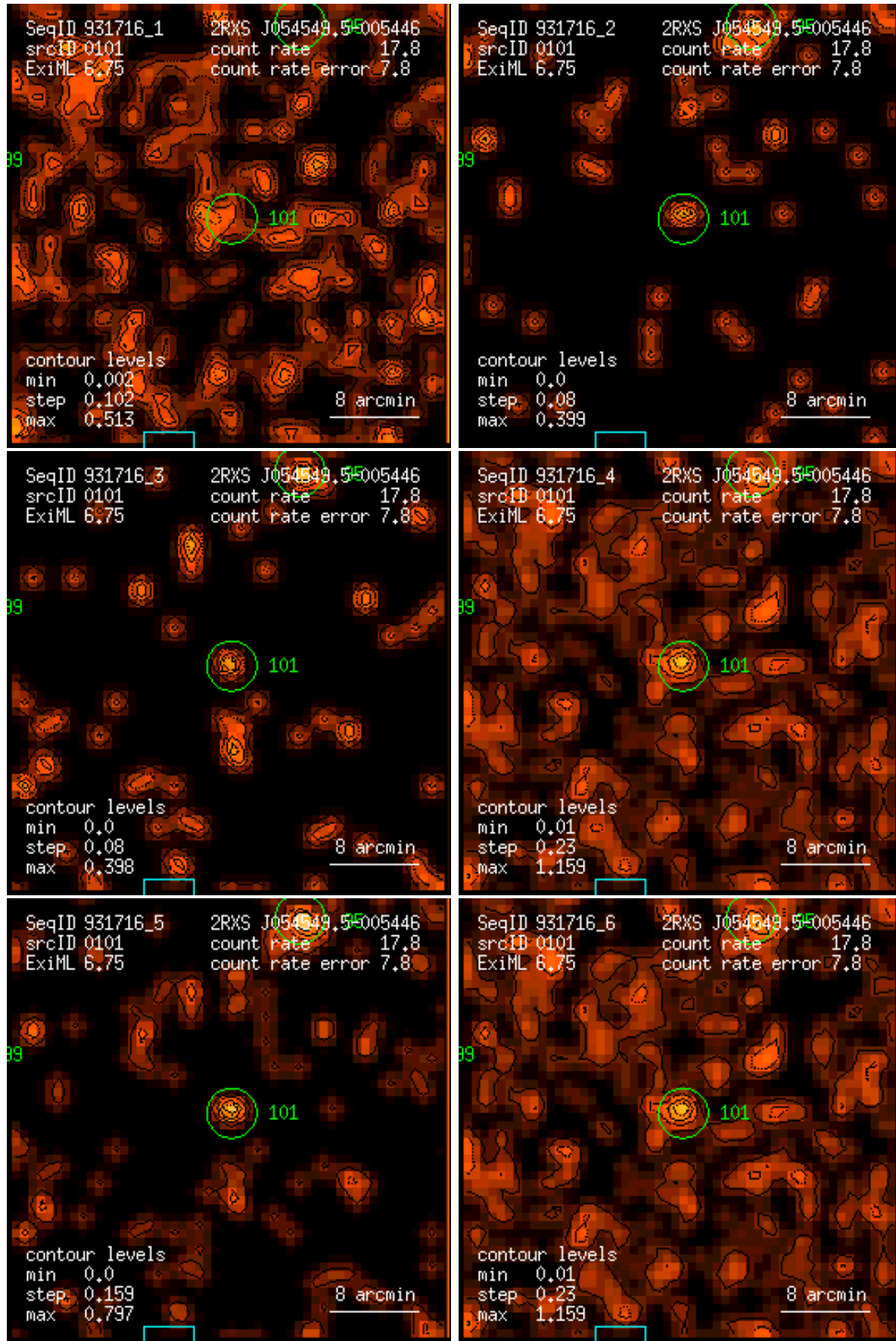
Figure 101: RASS 931716: detection 0101: band rate images, Gaussian filter: (1) PSPC channels 11 – 41, (2) 52 – 90, (3) 91 – 201, (4) 11 – 235, (5) 52 – 201, (6) 11 – 201. Broad band rates in counts/ks. Band rate contour levels in counts/ks/arcmin 2 .
