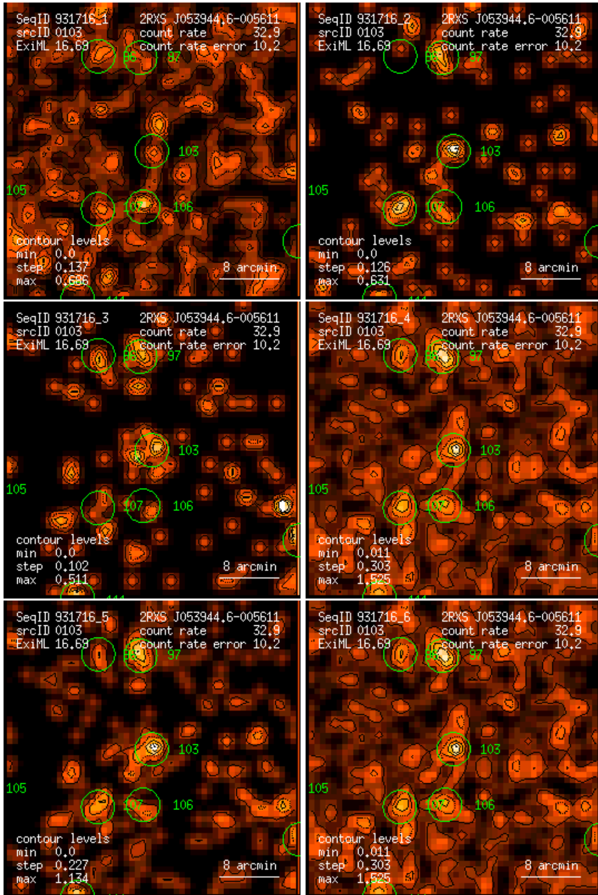
Figure 103: RASS 931716: detection 0103: band rate images, Gaussian filter: (1) PSPC channels 11 – 41, (2) 52 – 90, (3) 91 – 201, (4) 11 – 235, (5) 52 – 201, (6) 11 – 201. Broad band rates in counts/ks. Band rate contour levels in counts/ks/arcmin 2 .
