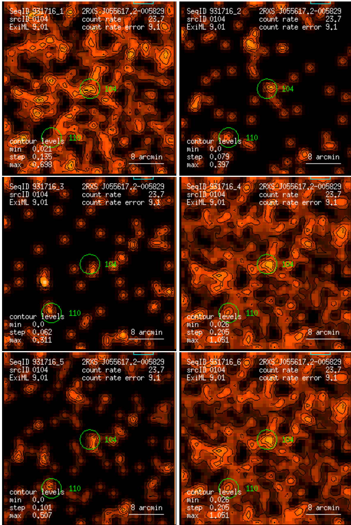
Figure 104: RASS 931716: detection 0104: band rate images, Gaussian filter: (1) PSPC channels 11 – 41, (2) 52 – 90, (3) 91 – 201, (4) 11 – 235, (5) 52 – 201, (6) 11 – 201. Broad band rates in counts/ks. Band rate contour levels in counts/ks/arcmin 2 .
