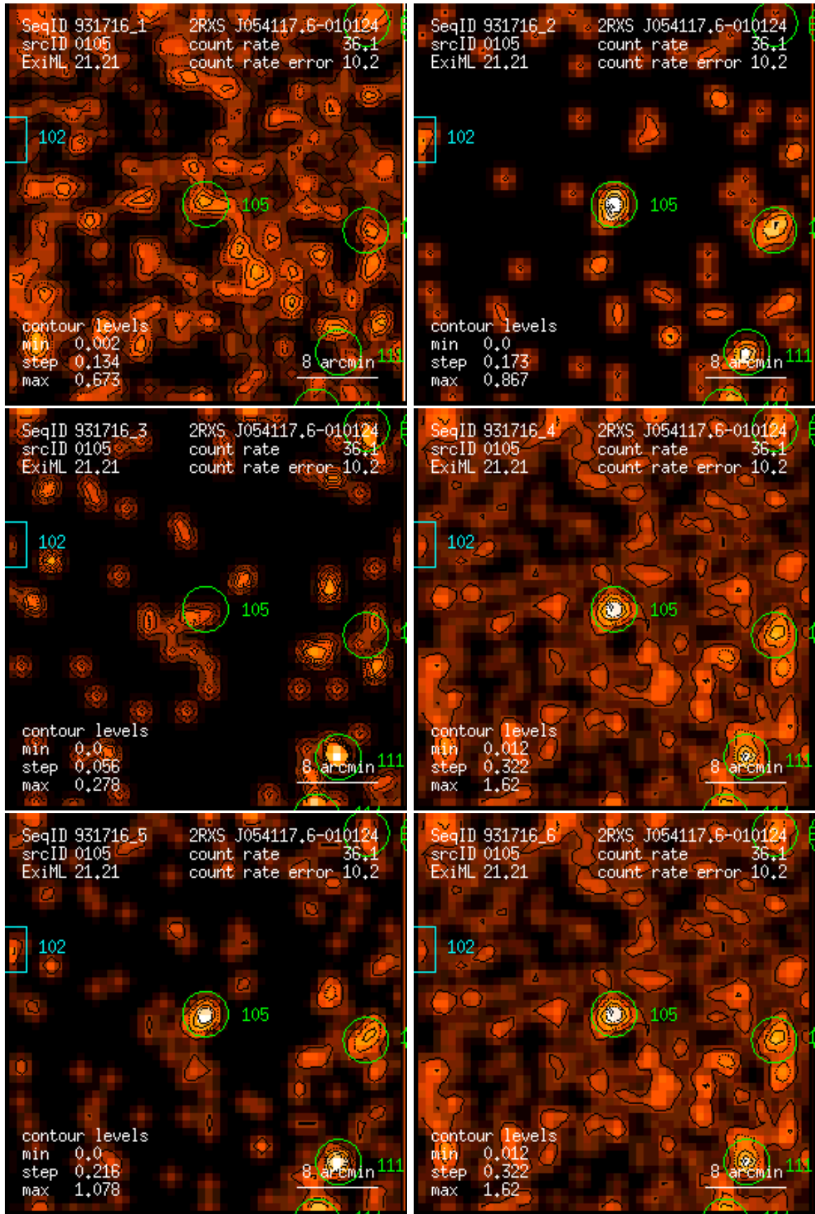
Figure 105: RASS 931716: detection 0105: band rate images, Gaussian filter: (1) PSPC channels 11 – 41, (2) 52 – 90, (3) 91 – 201, (4) 11 – 235, (5) 52 – 201, (6) 11 – 201. Broad band rates in counts/ks. Band rate contour levels in counts/ks/arcmin 2 .
