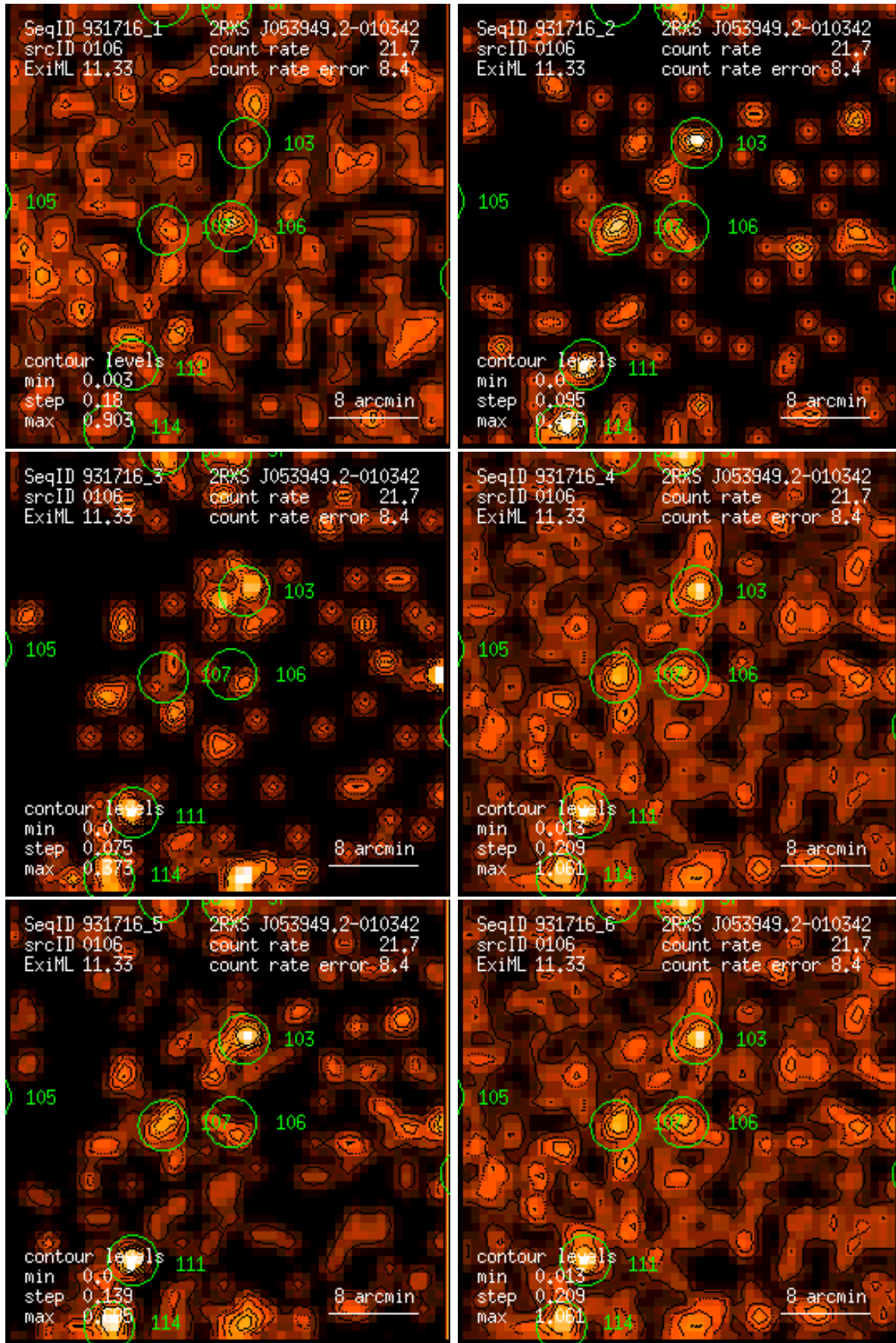
Figure 106: RASS 931716: detection 0106: band rate images, Gaussian filter: (1) PSPC channels 11 – 41, (2) 52 – 90, (3) 91 – 201, (4) 11 – 235, (5) 52 – 201, (6) 11 – 201. Broad band rates in counts/ks. Band rate contour levels in counts/ks/arcmin 2 .
