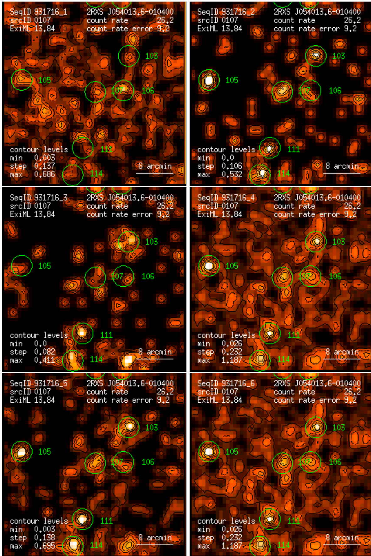
Figure 107: RASS 931716: detection 0107: band rate images, Gaussian filter: (1) PSPC channels 11 – 41, (2) 52 – 90, (3) 91 – 201, (4) 11 – 235, (5) 52 – 201, (6) 11 – 201. Broad band rates in counts/ks. Band rate contour levels in counts/ks/arcmin 2 .
