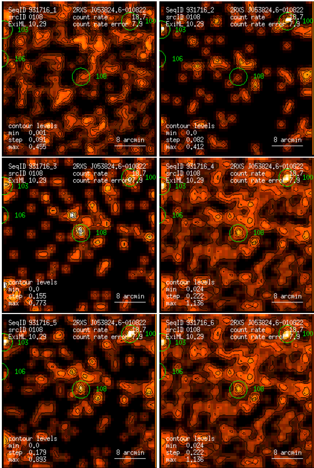
Figure 108: RASS 931716: detection 0108: band rate images, Gaussian filter: (1) PSPC channels 11 – 41, (2) 52 – 90, (3) 91 – 201, (4) 11 – 235, (5) 52 – 201, (6) 11 – 201. Broad band rates in counts/ks. Band rate contour levels in counts/ks/arcmin 2 .
