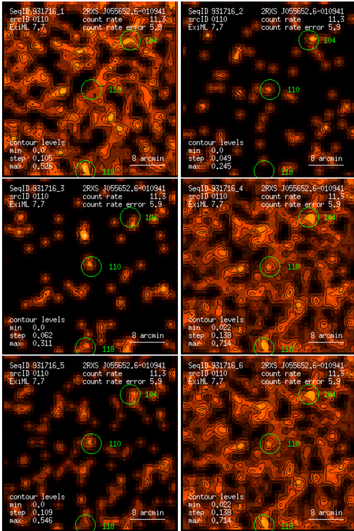
Figure 110: RASS 931716: detection 0110: band rate images, Gaussian filter: (1) PSPC channels 11 – 41, (2) 52 – 90, (3) 91 – 201, (4) 11 – 235, (5) 52 – 201, (6) 11 – 201. Broad band rates in counts/ks. Band rate contour levels in counts/ks/arcmin 2 .
