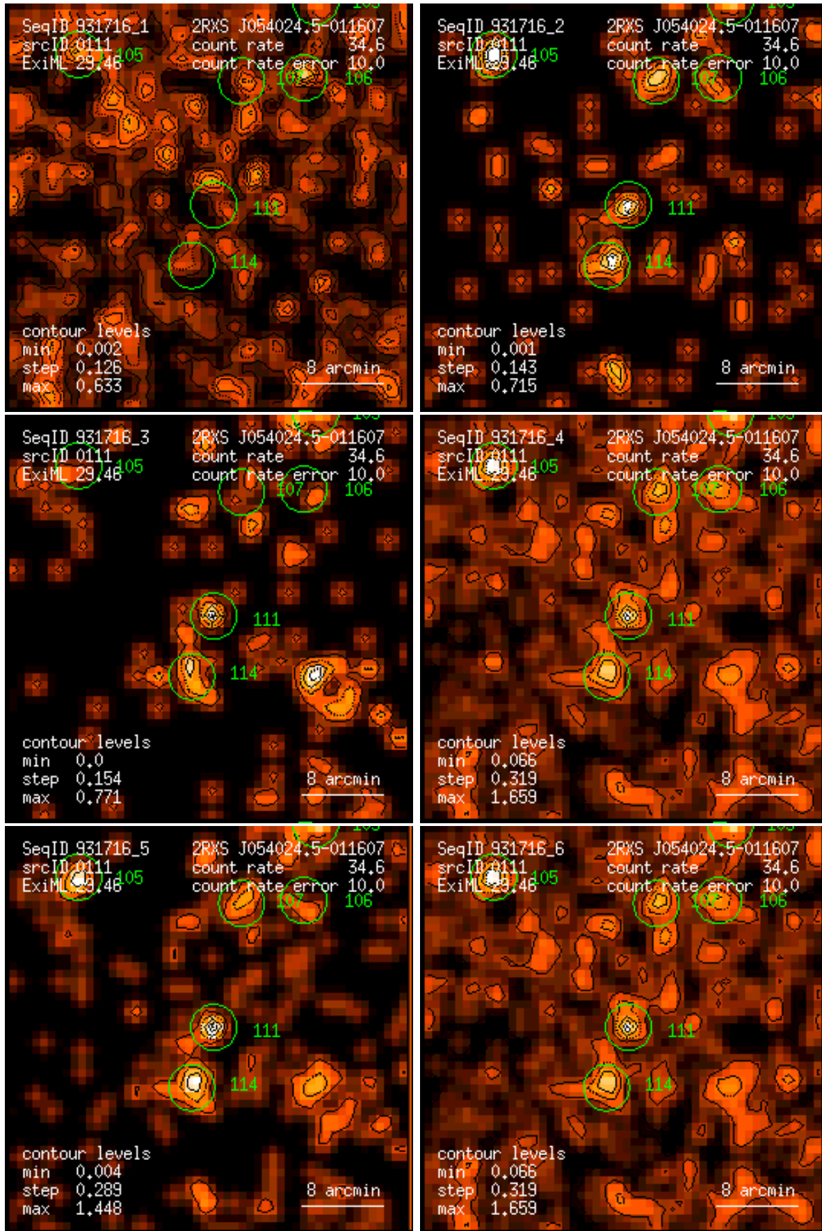
Figure 111: RASS 931716: detection 0111: band rate images, Gaussian filter: (1) PSPC channels 11 – 41, (2) 52 – 90, (3) 91 – 201, (4) 11 – 235, (5) 52 – 201, (6) 11 – 201. Broad band rates in counts/ks. Band rate contour levels in counts/ks/arcmin 2 .
