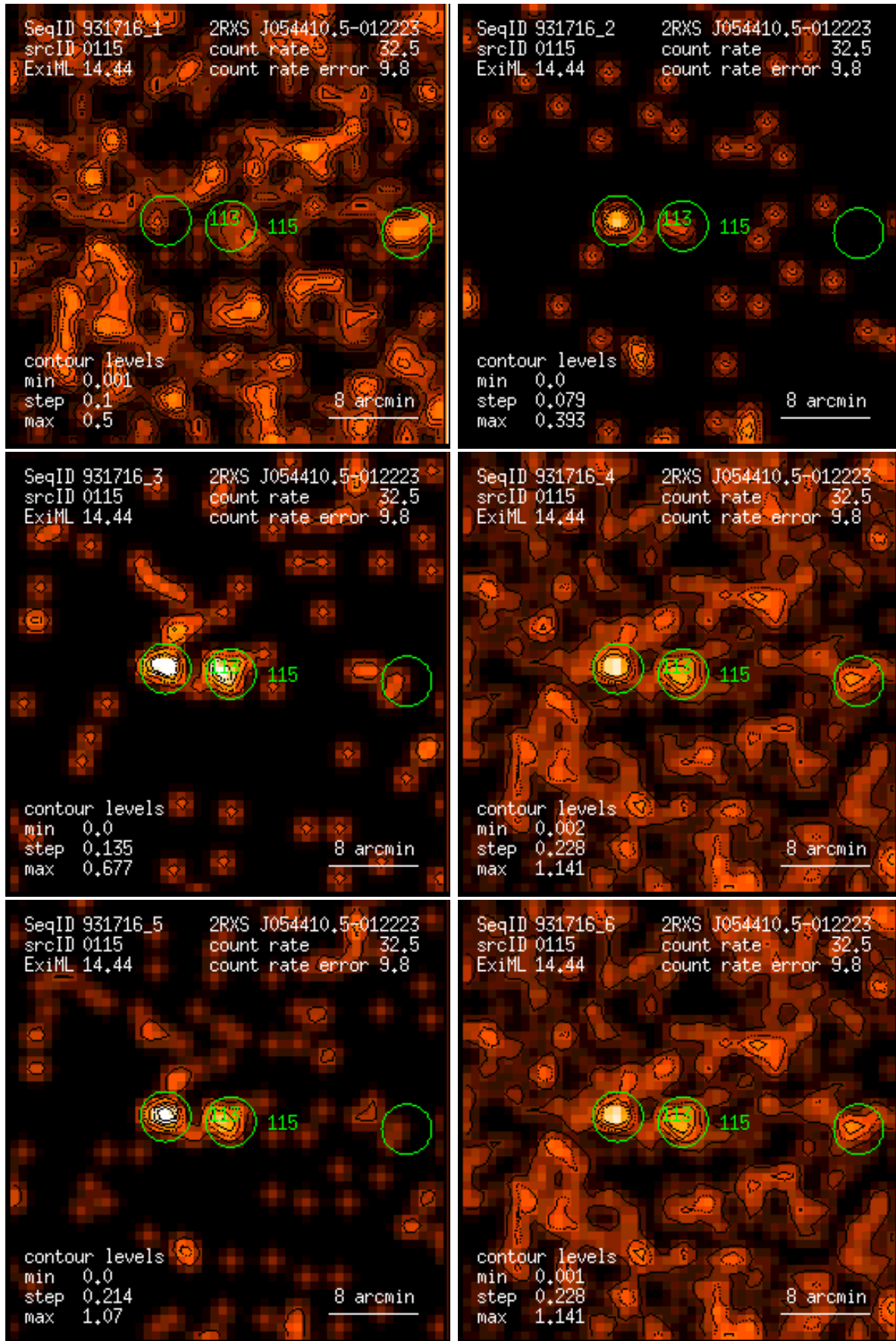
Figure 115: RASS 931716: detection 0115: band rate images, Gaussian filter: (1) PSPC channels 11 – 41, (2) 52 – 90, (3) 91 – 201, (4) 11 – 235, (5) 52 – 201, (6) 11 – 201. Broad band rates in counts/ks. Band rate contour levels in counts/ks/arcmin 2 .
