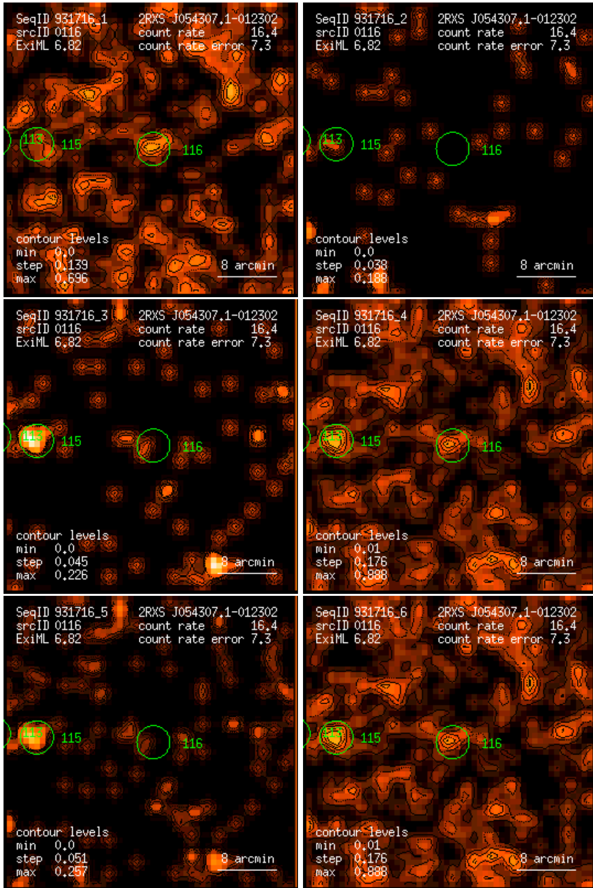
Figure 116: RASS 931716: detection 0116: band rate images, Gaussian filter: (1) PSPC channels 11 – 41, (2) 52 – 90, (3) 91 – 201, (4) 11 – 235, (5) 52 – 201, (6) 11 – 201. Broad band rates in counts/ks. Band rate contour levels in counts/ks/arcmin 2 .
