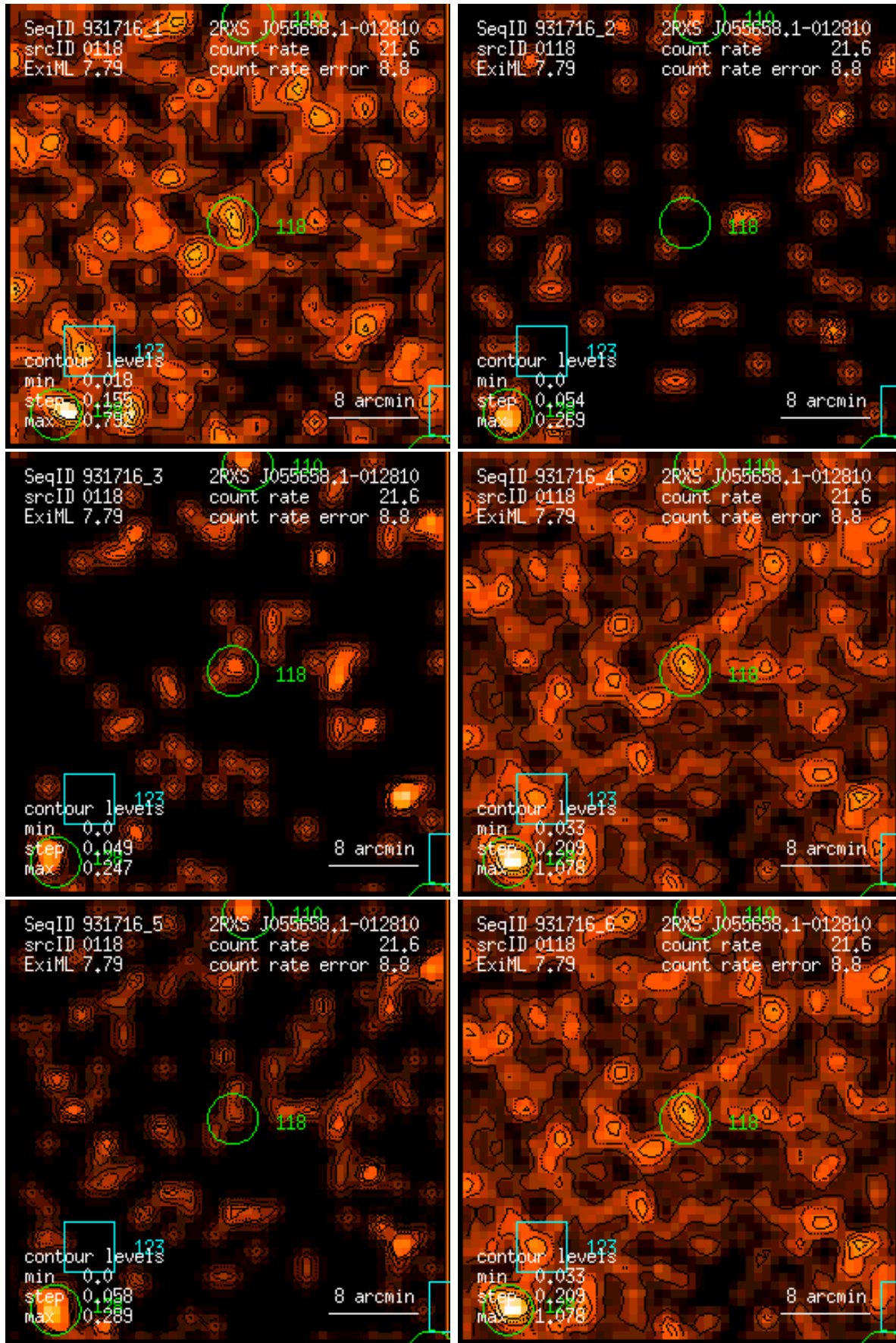
Figure 118: RASS 931716: detection 0118: band rate images, Gaussian filter: (1) PSPC channels 11 – 41, (2) 52 – 90, (3) 91 – 201, (4) 11 – 235, (5) 52 – 201, (6) 11 – 201. Broad band rates in counts/ks. Band rate contour levels in counts/ks/arcmin 2 .
