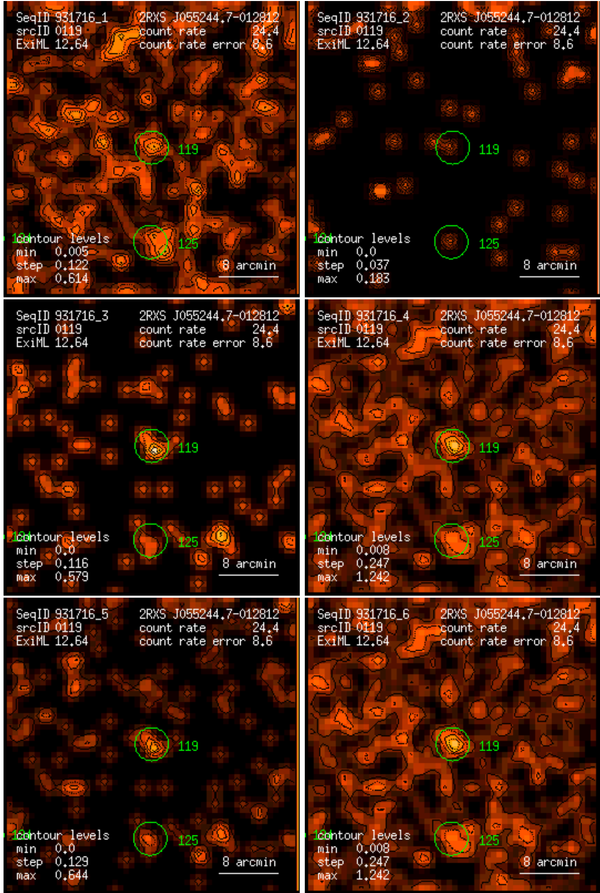
Figure 119: RASS 931716: detection 0119: band rate images, Gaussian filter: (1) PSPC channels 11 – 41, (2) 52 – 90, (3) 91 – 201, (4) 11 – 235, (5) 52 – 201, (6) 11 – 201. Broad band rates in counts/ks. Band rate contour levels in counts/ks/arcmin 2 .
