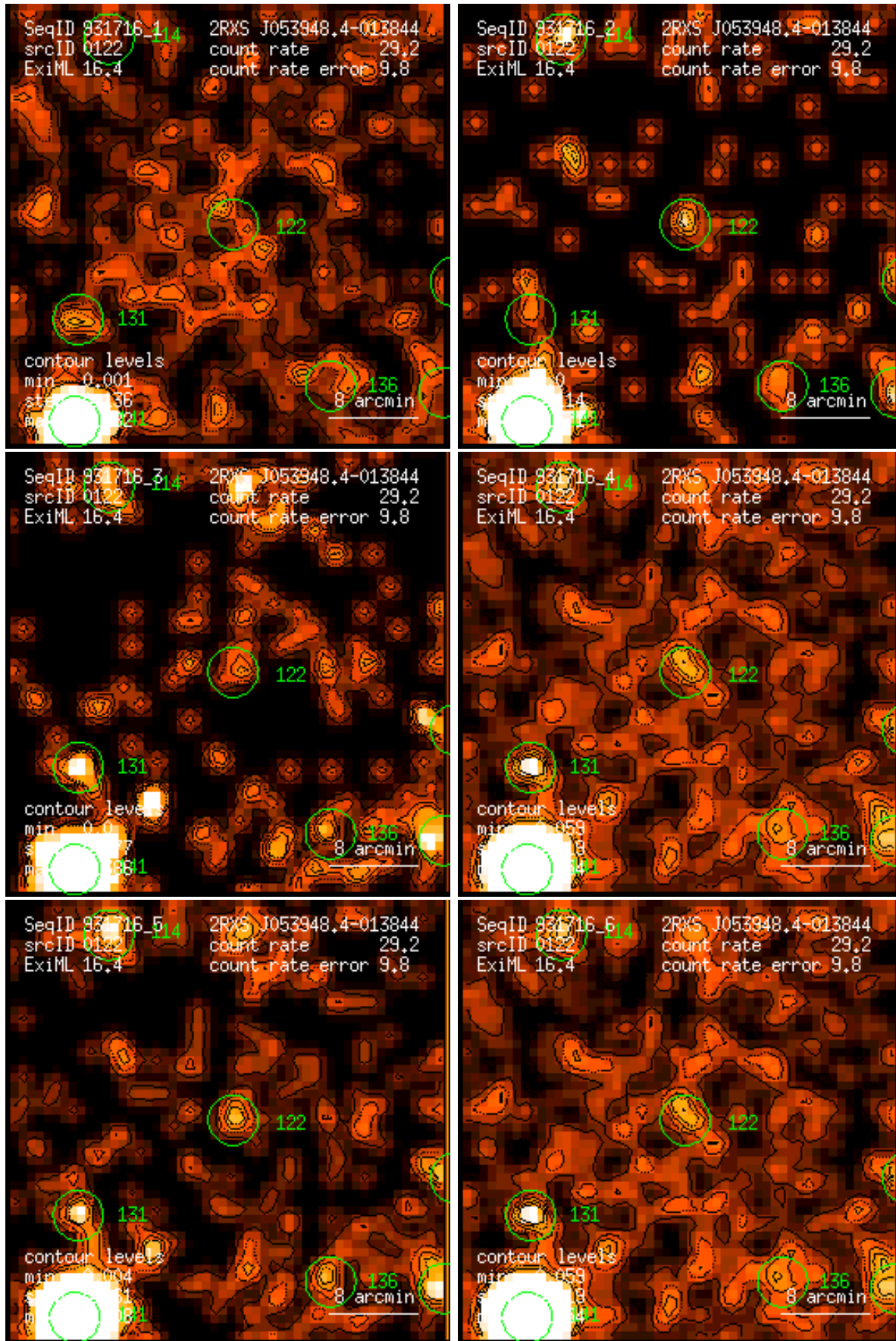
Figure 122: RASS 931716: detection 0122: band rate images, Gaussian filter: (1) PSPC channels 11 – 41, (2) 52 – 90, (3) 91 – 201, (4) 11 – 235, (5) 52 – 201, (6) 11 – 201. Broad band rates in counts/ks. Band rate contour levels in counts/ks/arcmin 2 .
