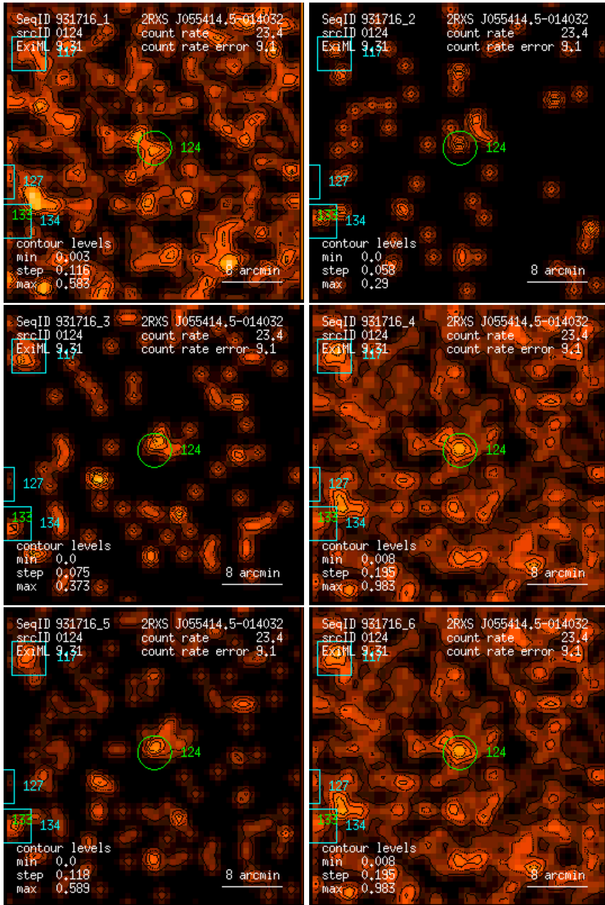
Figure 124: RASS 931716: detection 0124: band rate images, Gaussian filter: (1) PSPC channels 11 – 41, (2) 52 – 90, (3) 91 – 201, (4) 11 – 235, (5) 52 – 201, (6) 11 – 201. Broad band rates in counts/ks. Band rate contour levels in counts/ks/arcmin 2 .
