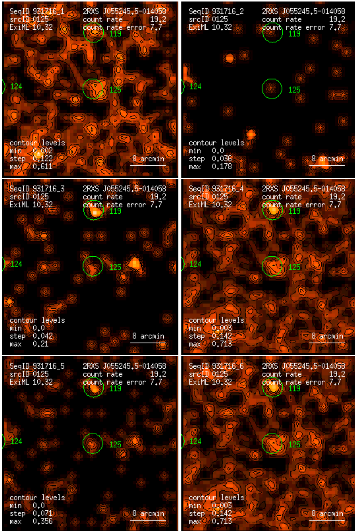
Figure 125: RASS 931716: detection 0125: band rate images, Gaussian filter: (1) PSPC channels 11 – 41, (2) 52 – 90, (3) 91 – 201, (4) 11 – 235, (5) 52 – 201, (6) 11 – 201. Broad band rates in counts/ks. Band rate contour levels in counts/ks/arcmin 2 .
