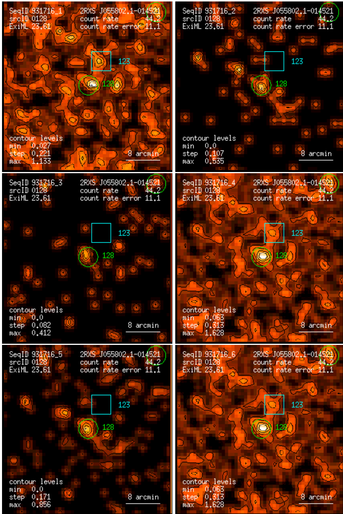
Figure 128: RASS 931716: detection 0128: band rate images, Gaussian filter: (1) PSPC channels 11 – 41, (2) 52 – 90, (3) 91 – 201, (4) 11 – 235, (5) 52 – 201, (6) 11 – 201. Broad band rates in counts/ks. Band rate contour levels in counts/ks/arcmin 2 .
