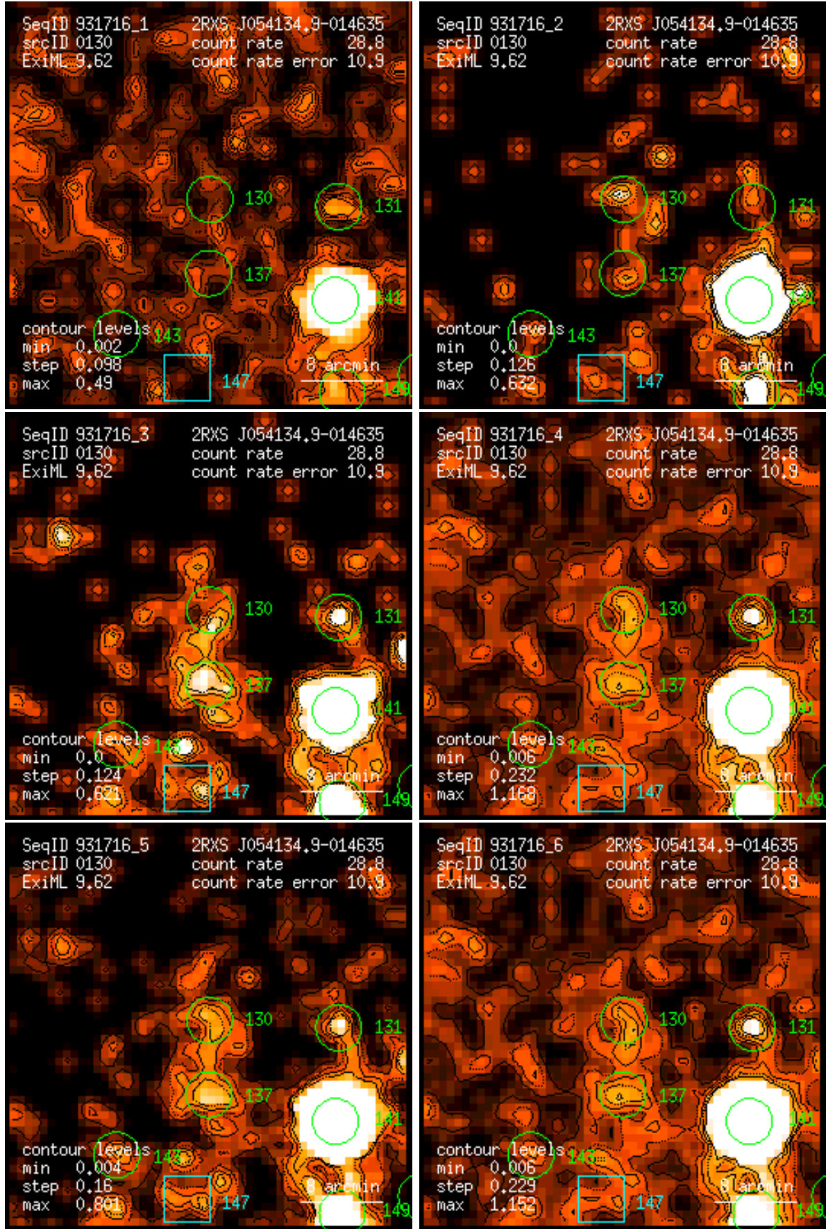
Figure 130: RASS 931716: detection 0130: band rate images, Gaussian filter: (1) PSPC channels 11 – 41, (2) 52 – 90, (3) 91 – 201, (4) 11 – 235, (5) 52 – 201, (6) 11 – 201. Broad band rates in counts/ks. Band rate contour levels in counts/ks/arcmin 2 .
