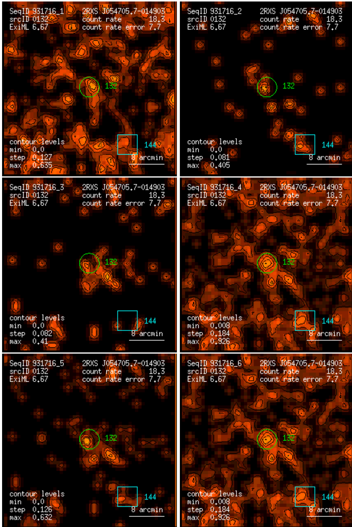
Figure 132: RASS 931716: detection 0132: band rate images, Gaussian filter: (1) PSPC channels 11 – 41, (2) 52 – 90, (3) 91 – 201, (4) 11 – 235, (5) 52 – 201, (6) 11 – 201. Broad band rates in counts/ks. Band rate contour levels in counts/ks/arcmin 2 .
