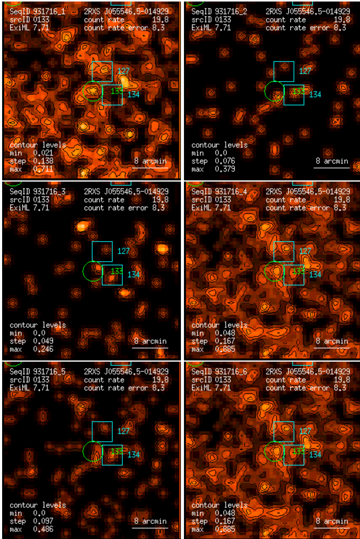
Figure 133: RASS 931716: detection 0133: band rate images, Gaussian filter: (1) PSPC channels 11 – 41, (2) 52 – 90, (3) 91 – 201, (4) 11 – 235, (5) 52 – 201, (6) 11 – 201. Broad band rates in counts/ks. Band rate contour levels in counts/ks/arcmin 2 .
