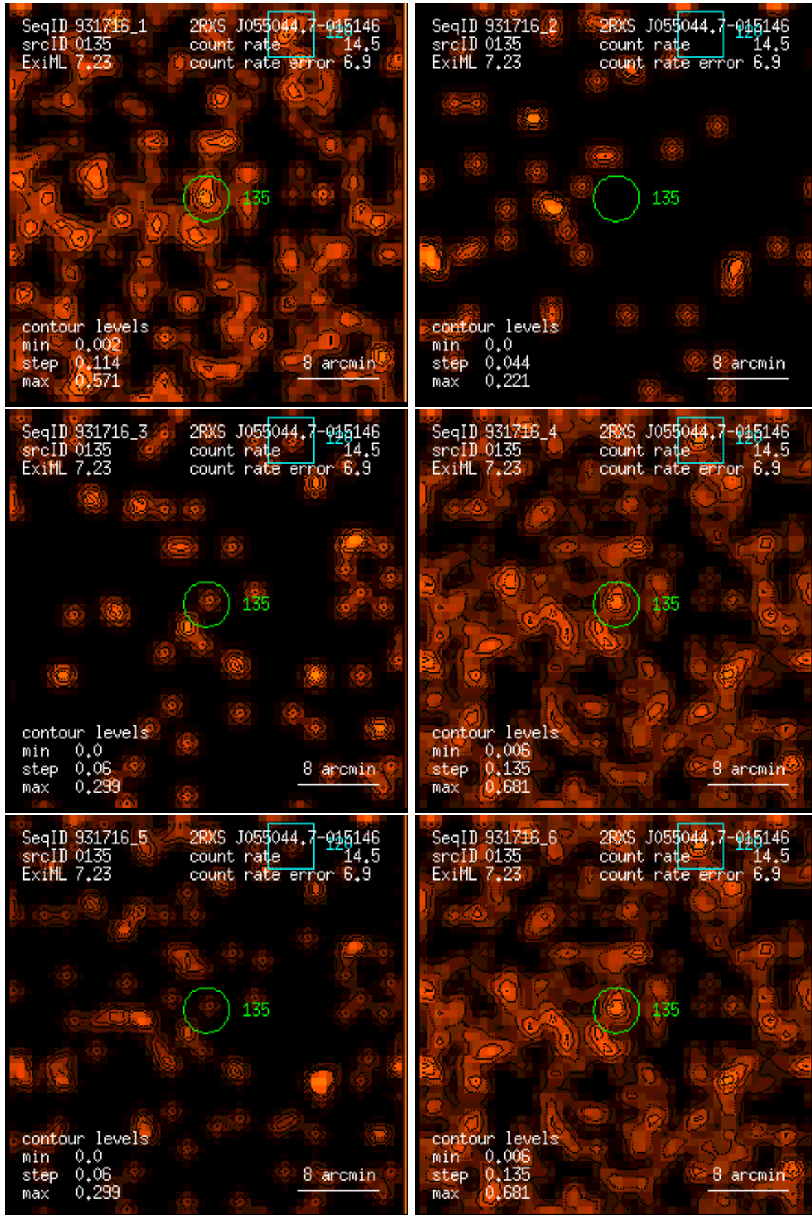
Figure 135: RASS 931716: detection 0135: band rate images, Gaussian filter: (1) PSPC channels 11 – 41, (2) 52 – 90, (3) 91 – 201, (4) 11 – 235, (5) 52 – 201, (6) 11 – 201. Broad band rates in counts/ks. Band rate contour levels in counts/ks/arcmin 2 .
