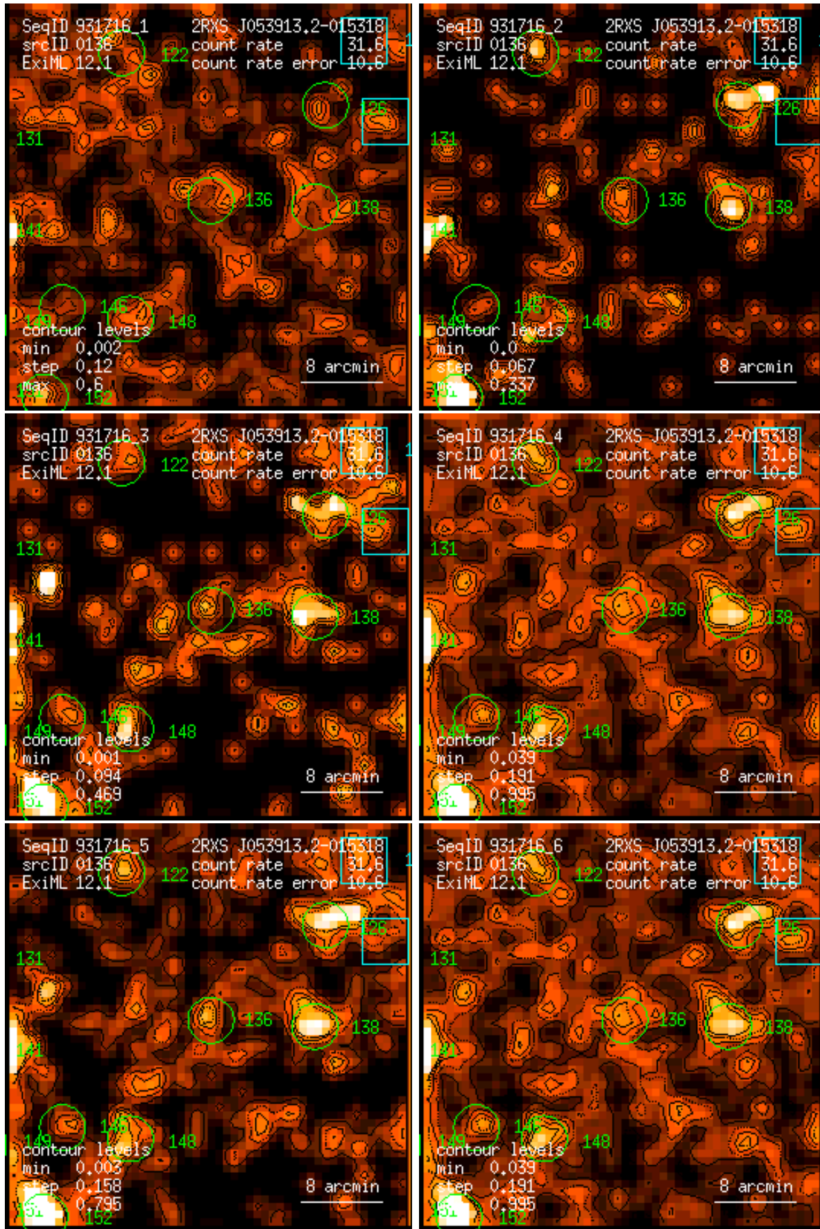
Figure 136: RASS 931716: detection 0136: band rate images, Gaussian filter: (1) PSPC channels 11 – 41, (2) 52 – 90, (3) 91 – 201, (4) 11 – 235, (5) 52 – 201, (6) 11 – 201. Broad band rates in counts/ks. Band rate contour levels in counts/ks/arcmin 2 .
