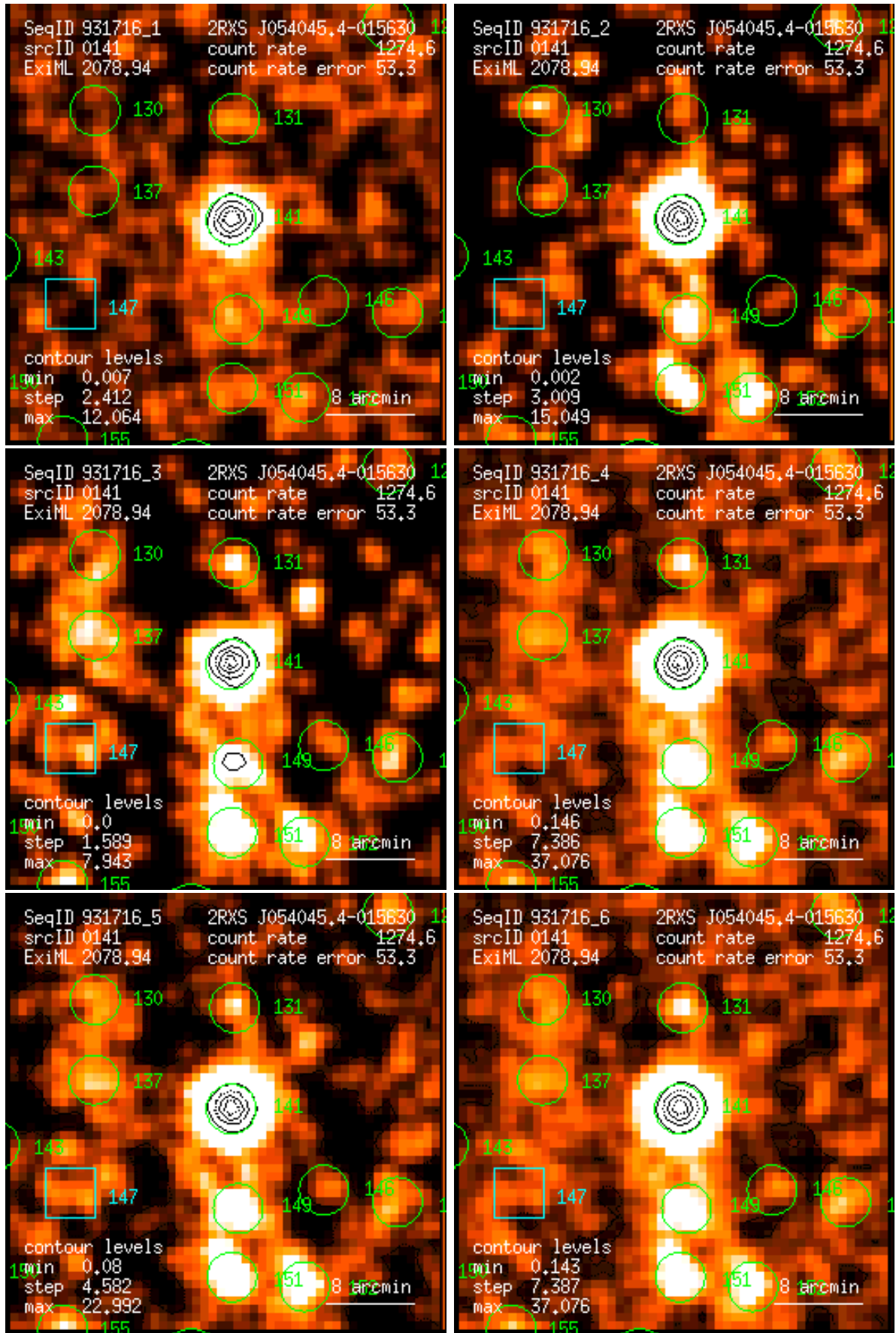
Figure 141: RASS 931716: detection 0141: band rate images, Gaussian filter: (1) PSPC channels 11 – 41, (2) 52 – 90, (3) 91 – 201, (4) 11 – 235, (5) 52 – 201, (6) 11 – 201. Broad band rates in counts/ks. Band rate contour levels in counts/ks/arcmin 2 .
