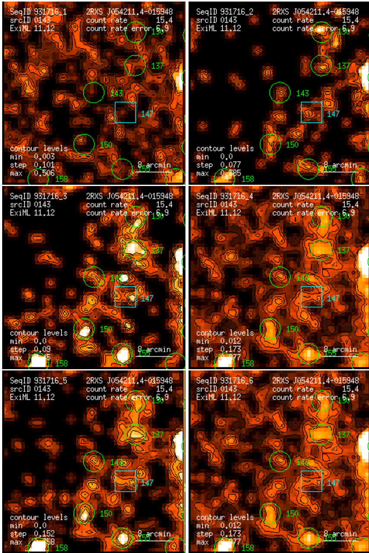
Figure 143: RASS 931716: detection 0143: band rate images, Gaussian filter: (1) PSPC channels 11 – 41, (2) 52 – 90, (3) 91 – 201, (4) 11 – 235, (5) 52 – 201, (6) 11 – 201. Broad band rates in counts/ks. Band rate contour levels in counts/ks/arcmin 2 .
