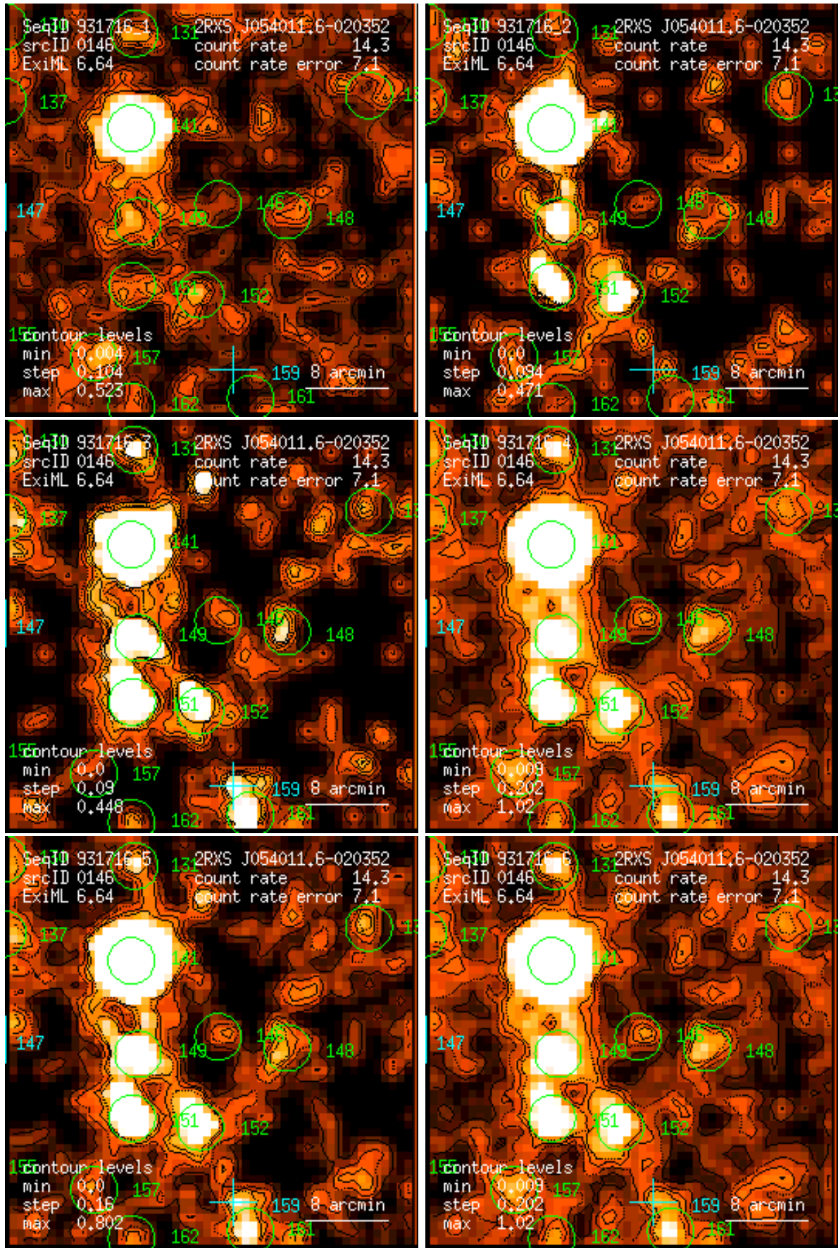
Figure 146: RASS 931716: detection 0146: band rate images, Gaussian filter: (1) PSPC channels 11 – 41, (2) 52 – 90, (3) 91 – 201, (4) 11 – 235, (5) 52 – 201, (6) 11 – 201. Broad band rates in counts/ks. Band rate contour levels in counts/ks/arcmin 2 .
