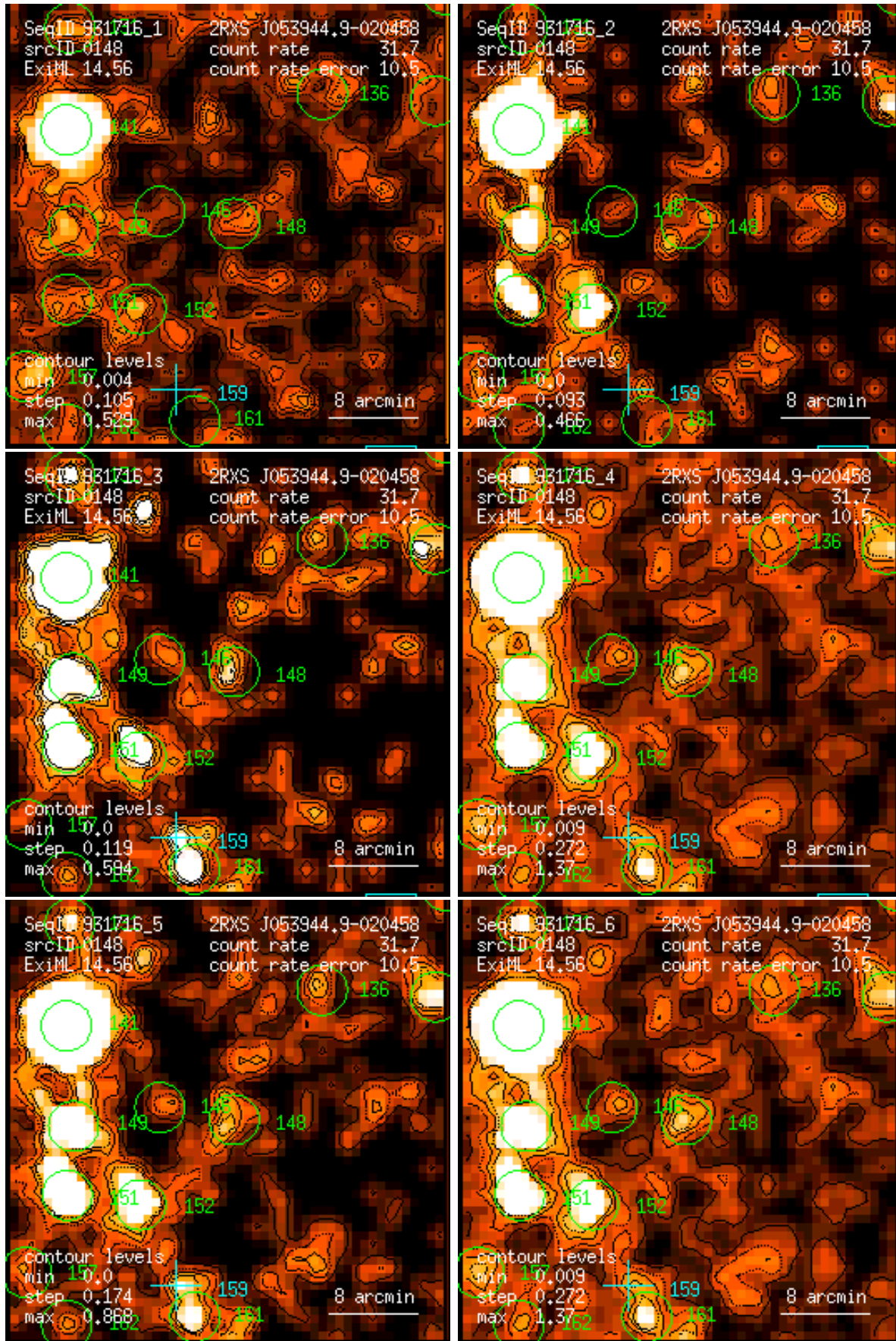
Figure 148: RASS 931716: detection 0148: band rate images, Gaussian filter: (1) PSPC channels 11 – 41, (2) 52 – 90, (3) 91 – 201, (4) 11 – 235, (5) 52 – 201, (6) 11 – 201. Broad band rates in counts/ks. Band rate contour levels in counts/ks/arcmin 2 .
