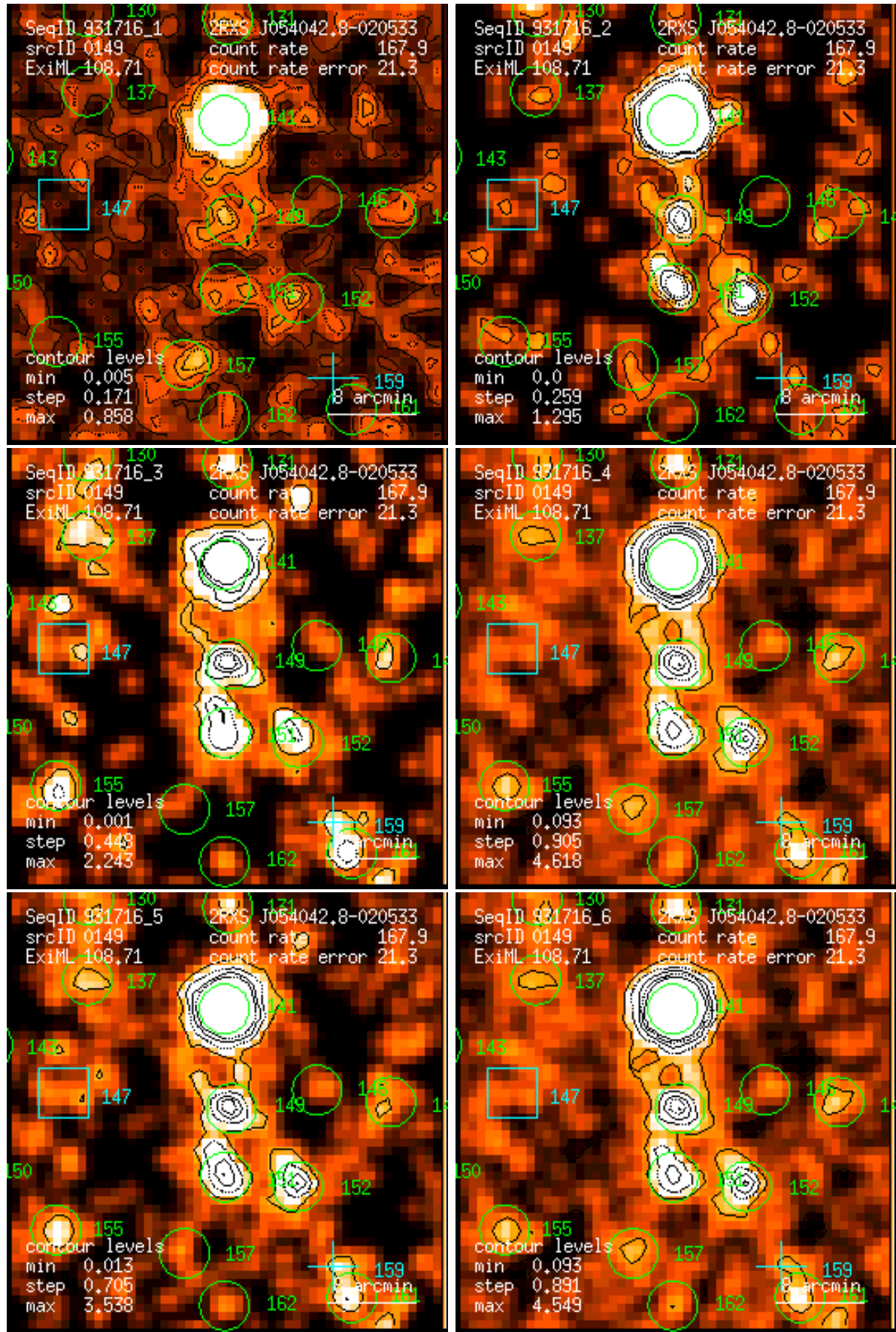
Figure 149: RASS 931716: detection 0149: band rate images, Gaussian filter: (1) PSPC channels 11 – 41, (2) 52 – 90, (3) 91 – 201, (4) 11 – 235, (5) 52 – 201, (6) 11 – 201. Broad band rates in counts/ks. Band rate contour levels in counts/ks/arcmin 2 .
