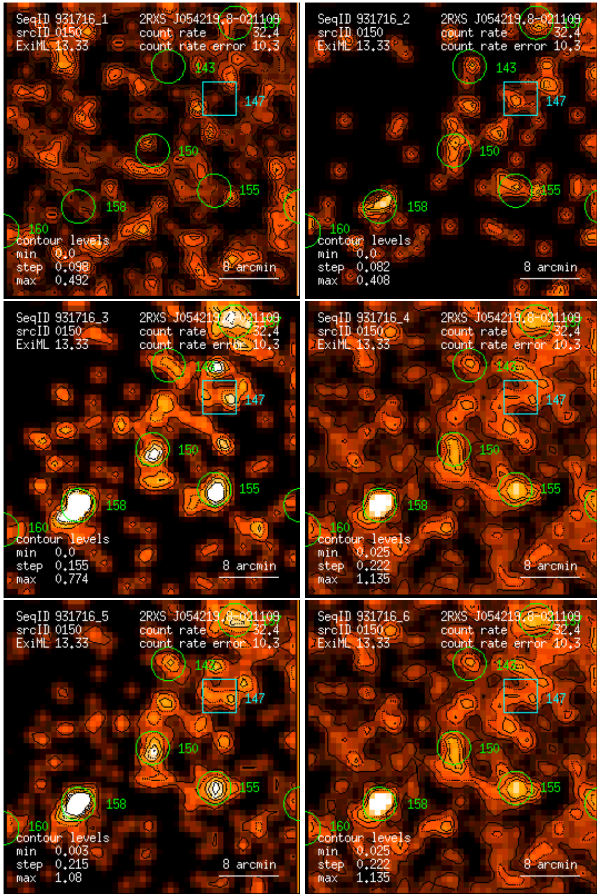
Figure 150: RASS 931716: detection 0150: band rate images, Gaussian filter: (1) PSPC channels 11 – 41, (2) 52 – 90, (3) 91 – 201, (4) 11 – 235, (5) 52 – 201, (6) 11 – 201. Broad band rates in counts/ks. Band rate contour levels in counts/ks/arcmin 2 .
