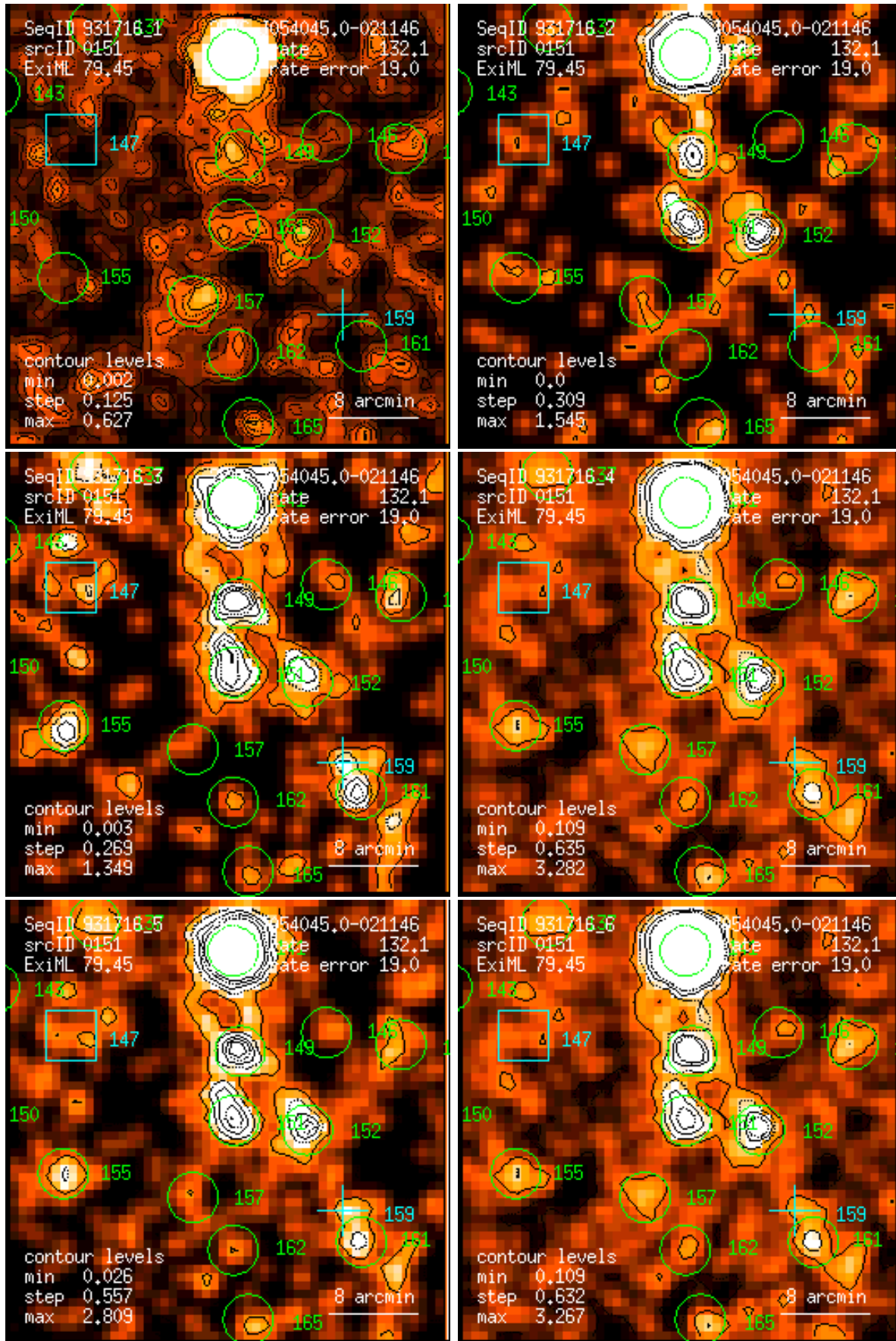
Figure 151: RASS 931716: detection 0151: band rate images, Gaussian filter: (1) PSPC channels 11 – 41, (2) 52 – 90, (3) 91 – 201, (4) 11 – 235, (5) 52 – 201, (6) 11 – 201. Broad band rates in counts/ks. Band rate contour levels in counts/ks/arcmin 2 .
