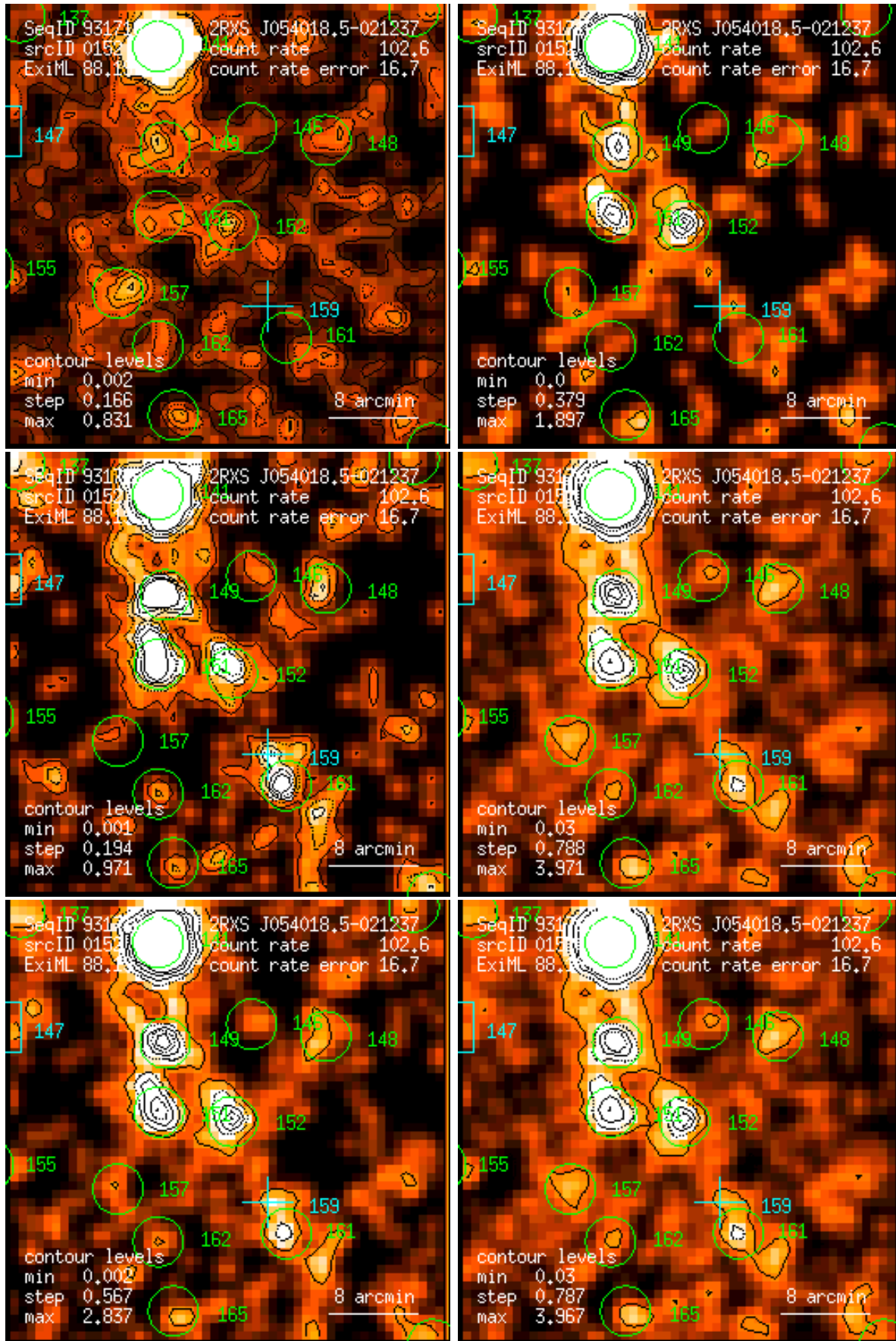
Figure 152: RASS 931716: detection 0152: band rate images, Gaussian filter: (1) PSPC channels 11 – 41, (2) 52 – 90, (3) 91 – 201, (4) 11 – 235, (5) 52 – 201, (6) 11 – 201. Broad band rates in counts/ks. Band rate contour levels in counts/ks/arcmin 2 .
