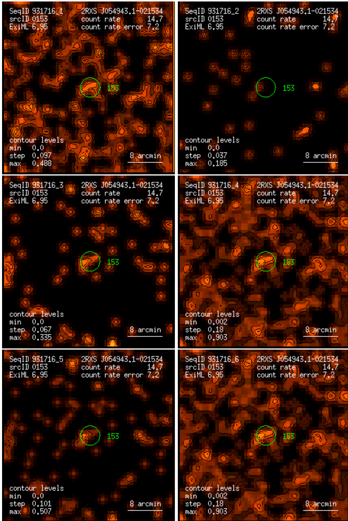
Figure 153: RASS 931716: detection 0153: band rate images, Gaussian filter: (1) PSPC channels 11 – 41, (2) 52 – 90, (3) 91 – 201, (4) 11 – 235, (5) 52 – 201, (6) 11 – 201. Broad band rates in counts/ks. Band rate contour levels in counts/ks/arcmin 2 .
