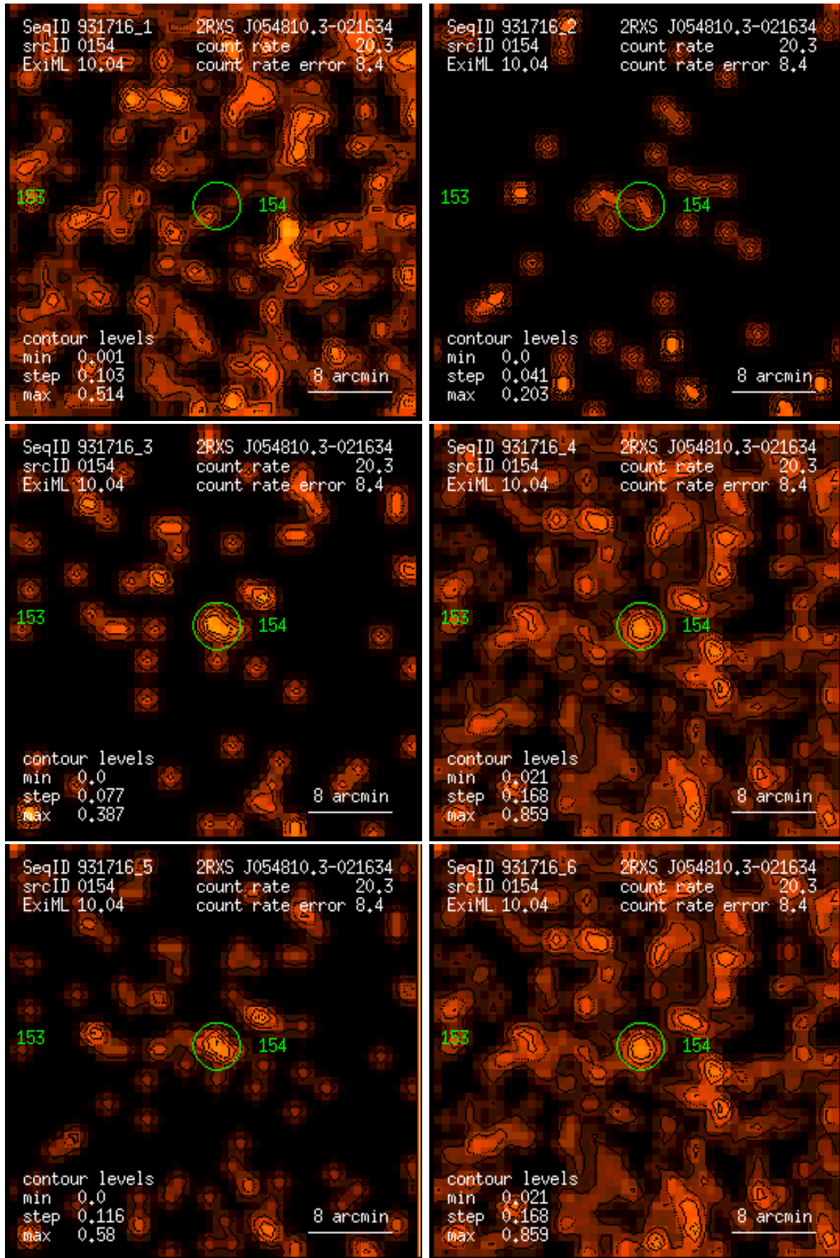
Figure 154: RASS 931716: detection 0154: band rate images, Gaussian filter: (1) PSPC channels 11 – 41, (2) 52 – 90, (3) 91 – 201, (4) 11 – 235, (5) 52 – 201, (6) 11 – 201. Broad band rates in counts/ks. Band rate contour levels in counts/ks/arcmin 2 .
