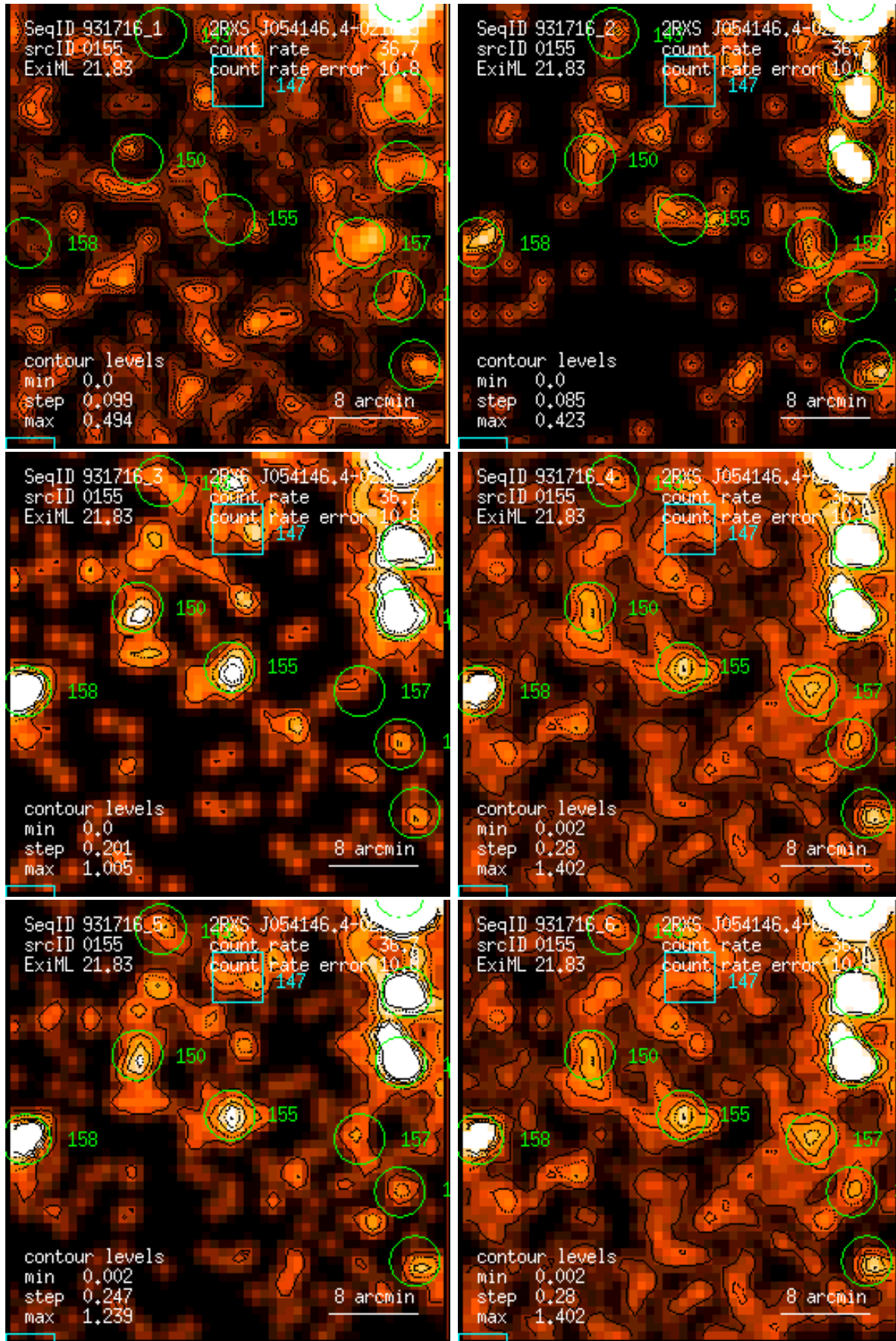
Figure 155: RASS 931716: detection 0155: band rate images, Gaussian filter: (1) PSPC channels 11 – 41, (2) 52 – 90, (3) 91 – 201, (4) 11 – 235, (5) 52 – 201, (6) 11 – 201. Broad band rates in counts/ks. Band rate contour levels in counts/ks/arcmin 2 .
