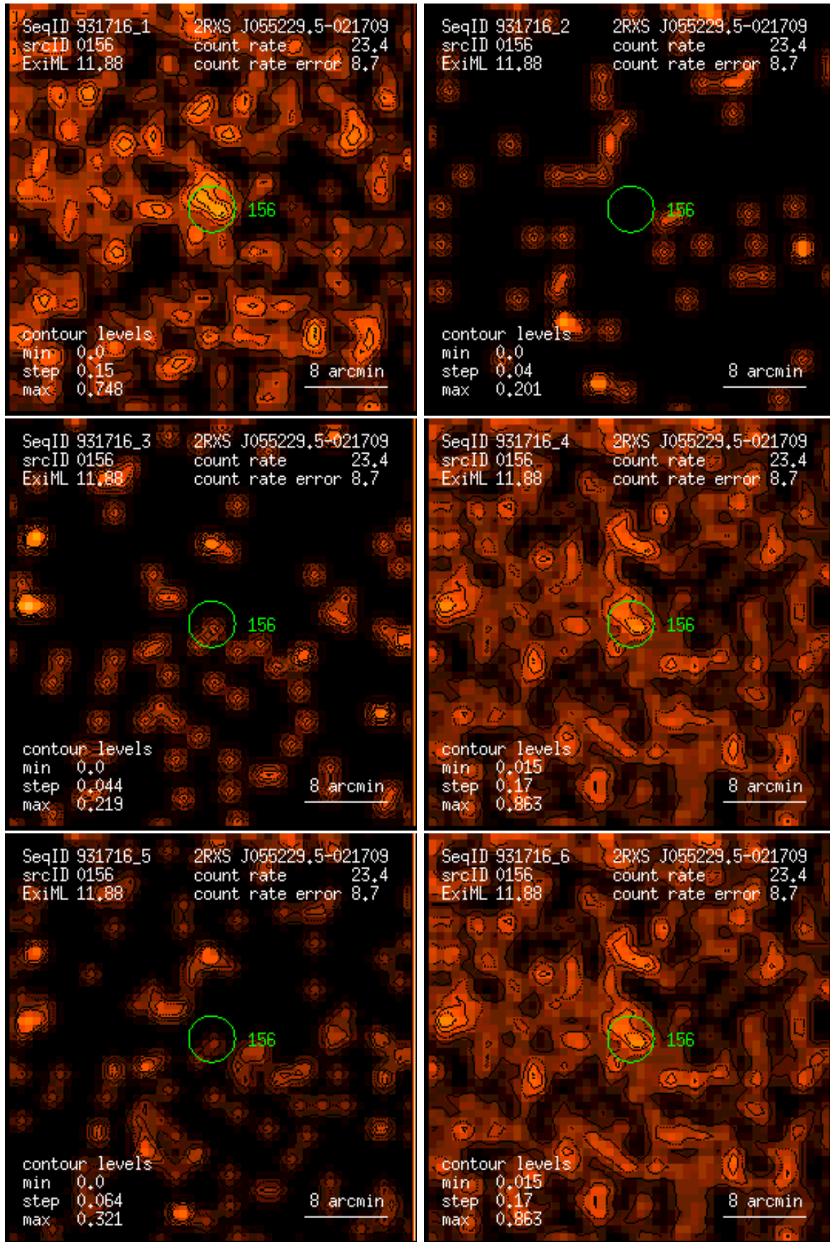
Figure 156: RASS 931716: detection 0156: band rate images, Gaussian filter: (1) PSPC channels 11 – 41, (2) 52 – 90, (3) 91 – 201, (4) 11 – 235, (5) 52 – 201, (6) 11 – 201. Broad band rates in counts/ks. Band rate contour levels in counts/ks/arcmin 2 .
